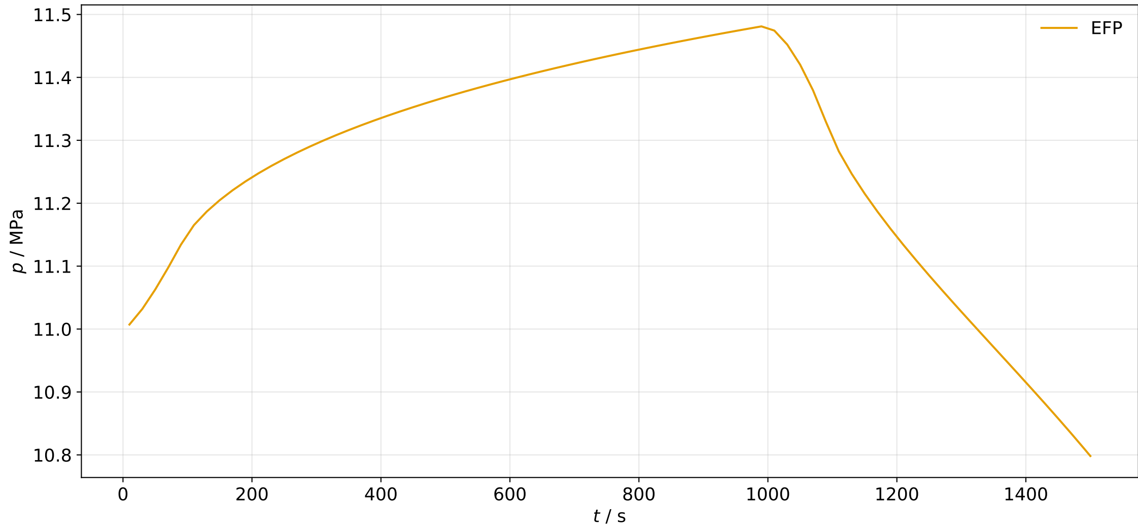
Pressure over Time at Bottom Inlet
