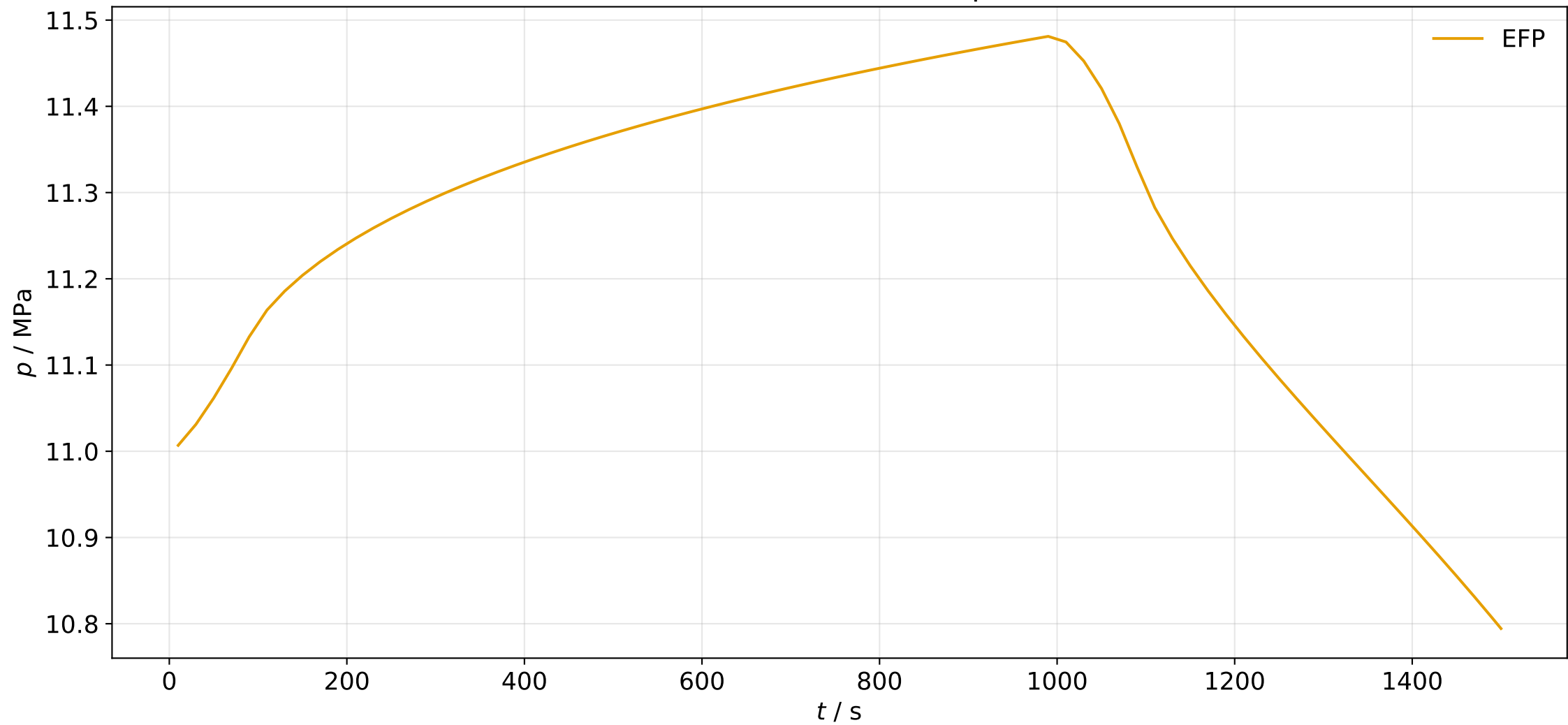
Pressure over Time at Top Inlet
