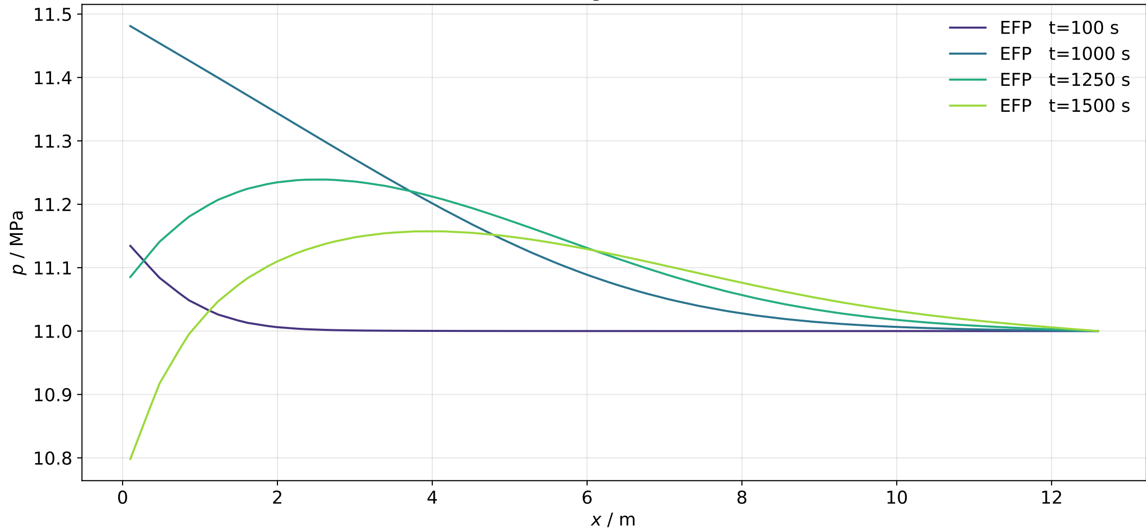
Pressure Along Bottom Fracture
