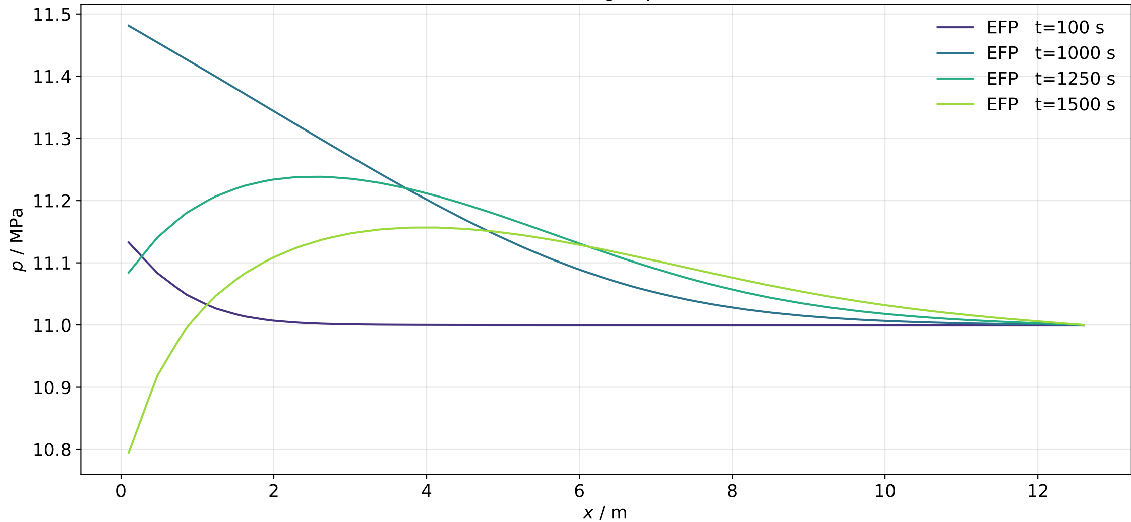
Pressure Along Top Fracture
