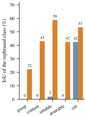
(b) Held-out question phrasing
