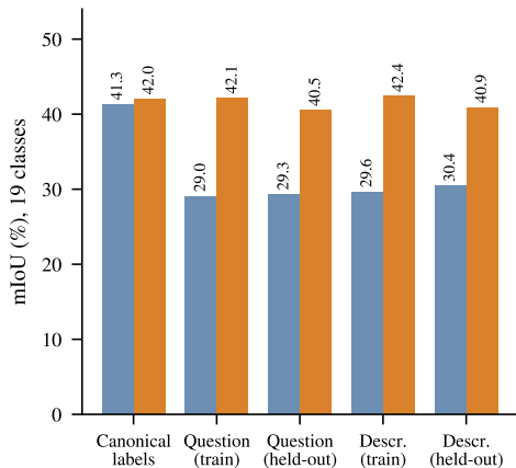
(a) Overall mIoU by phrasing condition
