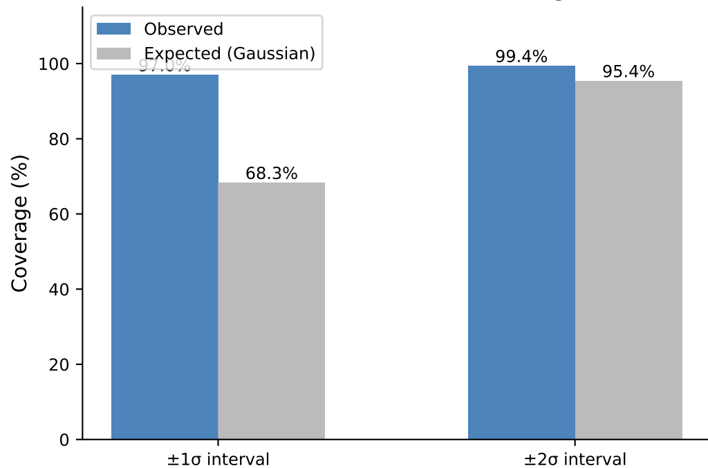
(b) Prediction Interval Coverage
