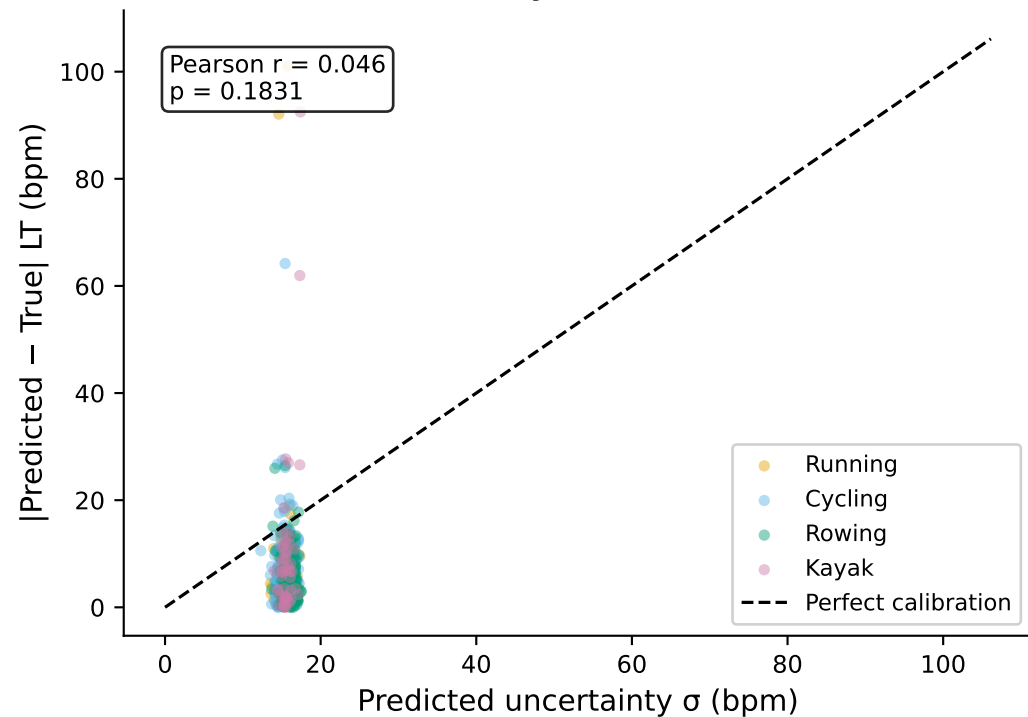
(a) Uncertainty vs. Absolute Error
