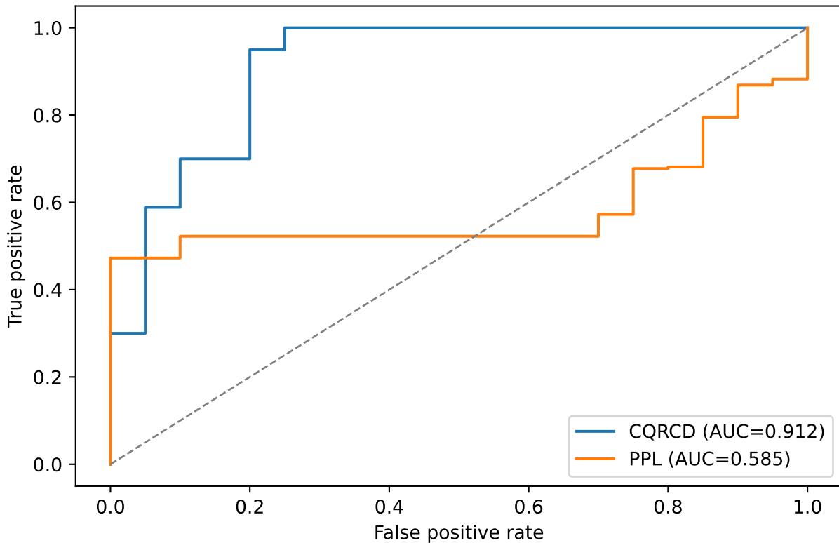
ROC comparison: CQRCD vs baselines
