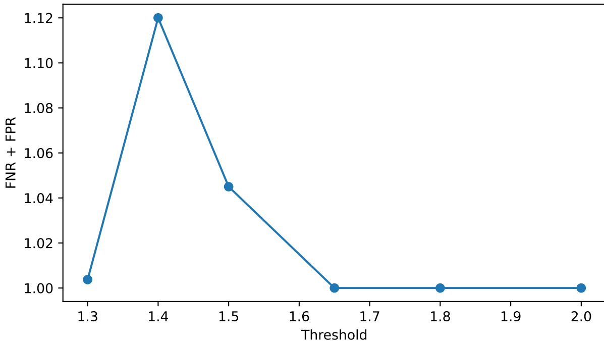
Ablation: threshold
