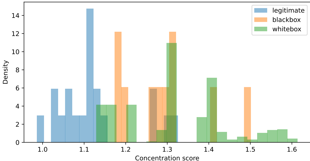
CQRCD concentration score distributions
