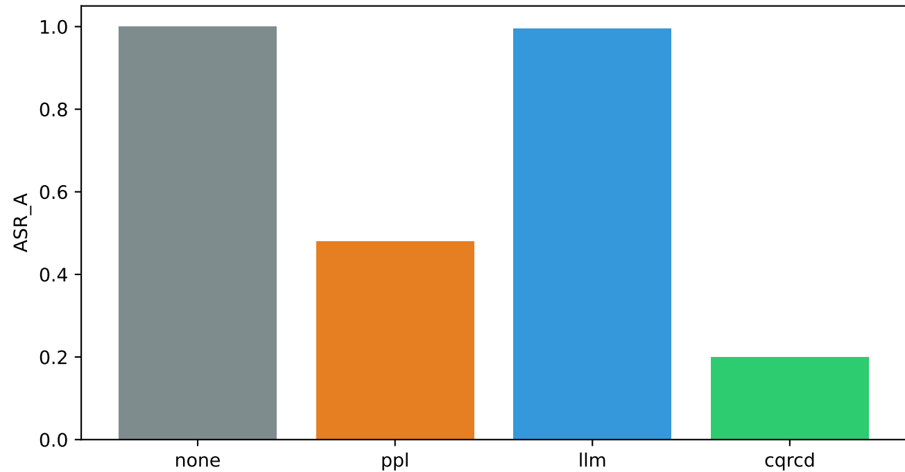
Attack success under defense conditions
