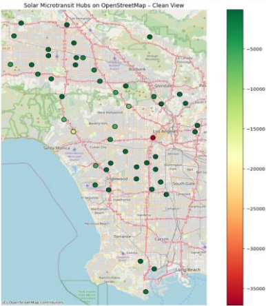
Fig. 3 — Net daily solar surplus/deficit by hub.
