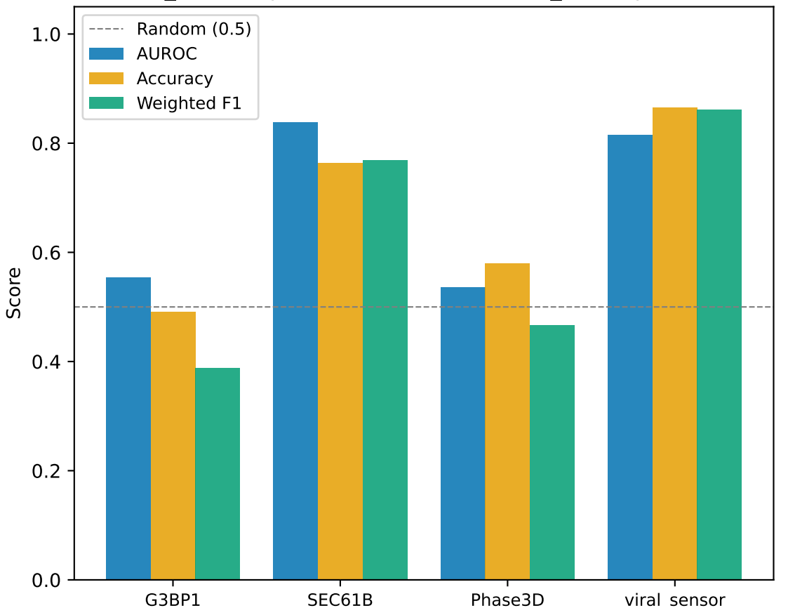
witness_state — performance vs infection_state (per marker)
