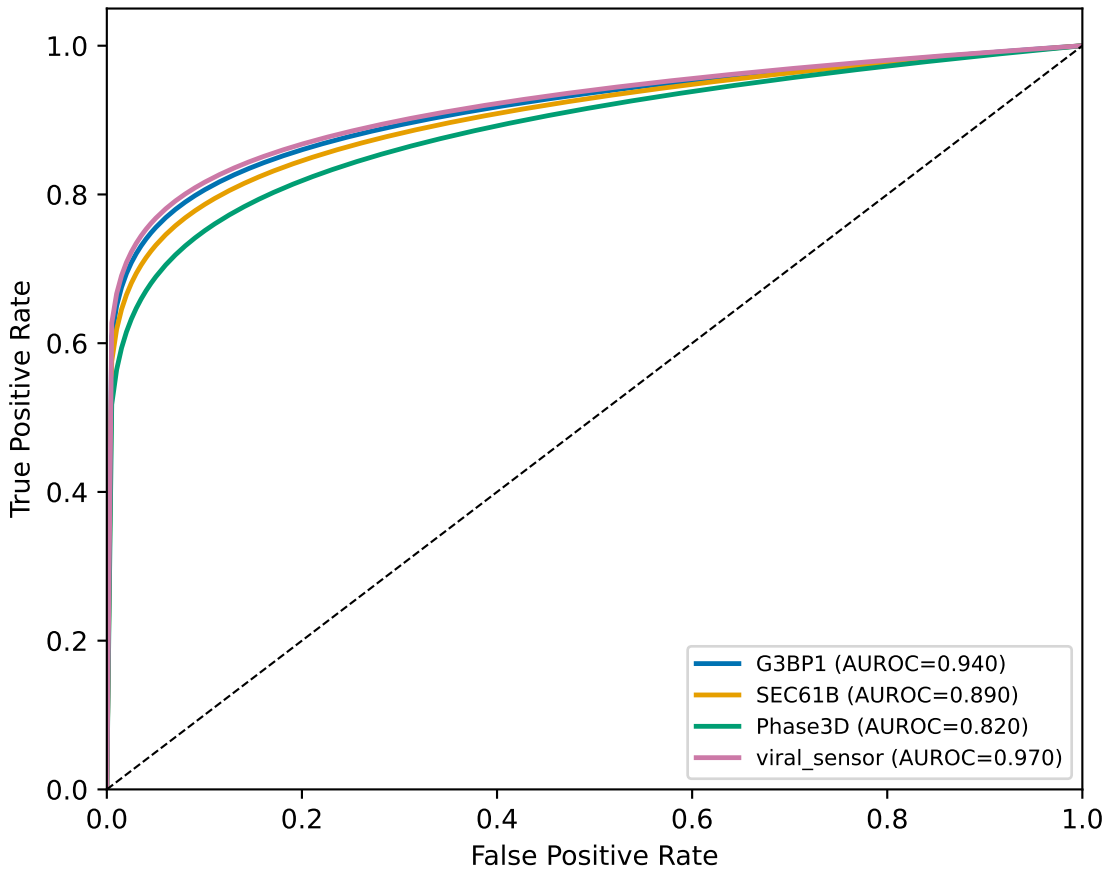
ROC — witness_state (per marker)
