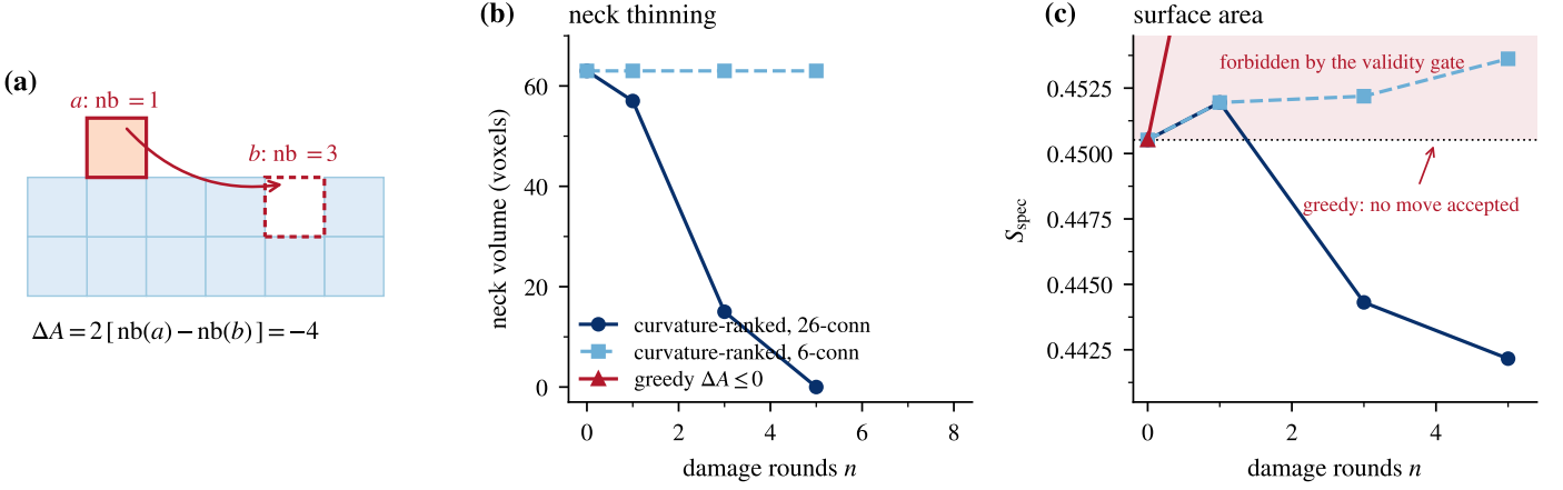
Figure 6: Two operators bracket an impossibility on a sphere-neck-sphere test body (neck 63 voxels, pristine S_{spec} = 0.45052 ). (a) The exact area change of one swap on a 6-connected lattice, Eq. (2): moving a voxel from a protrusion to a notch lowers exposed area by four faces. (b) Neck volume. The curvature-ranked operator with a 26-connectivity stencil thins the neck to zero; with 6-connectivity it does nothing; the greedy operator leaves the neck intact. (c) Surface area. The curvature-ranked operator enters the region forbidden by its own validity criterion at n = 1 , at 0.45195 against a pristine 0.45052, before falling below pristine at n = 3 . The greedy operator accepts 96% of proposals and also rises above pristine, to 0.46365 at n = 1 , because per-move \Delta A \leq 0 guarantees do not compose across a batch ranked on a stale neighbour field. Data: o5v2_area_barrier.csv , regenerated by o5v2_regenerate.py .
