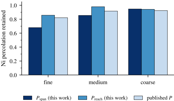
(a) Fine retains Ni percolation worst
