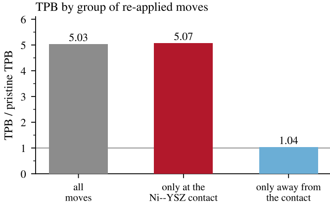
Figure 9: Where the triple-line inflation comes from, by re-applying the two groups of moves separately to the pristine structure. Moves that touch the nickel–zirconia contact reproduce the whole artifact on their own; every other move, 97 % of the added material, changes TPB by four percent. Data: o7_counterfactual.csv .
