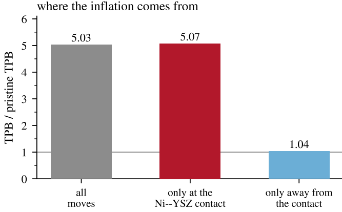
Figure 8: Where the triple-line inflation comes from, by re-applying the two groups of moves separately to the pristine structure. Moves that touch the nickel–zirconia contact reproduce the whole artifact on their own; every other move, 97 % of the added material, changes TPB by four percent. Data: o7_counterfactual.csv .
