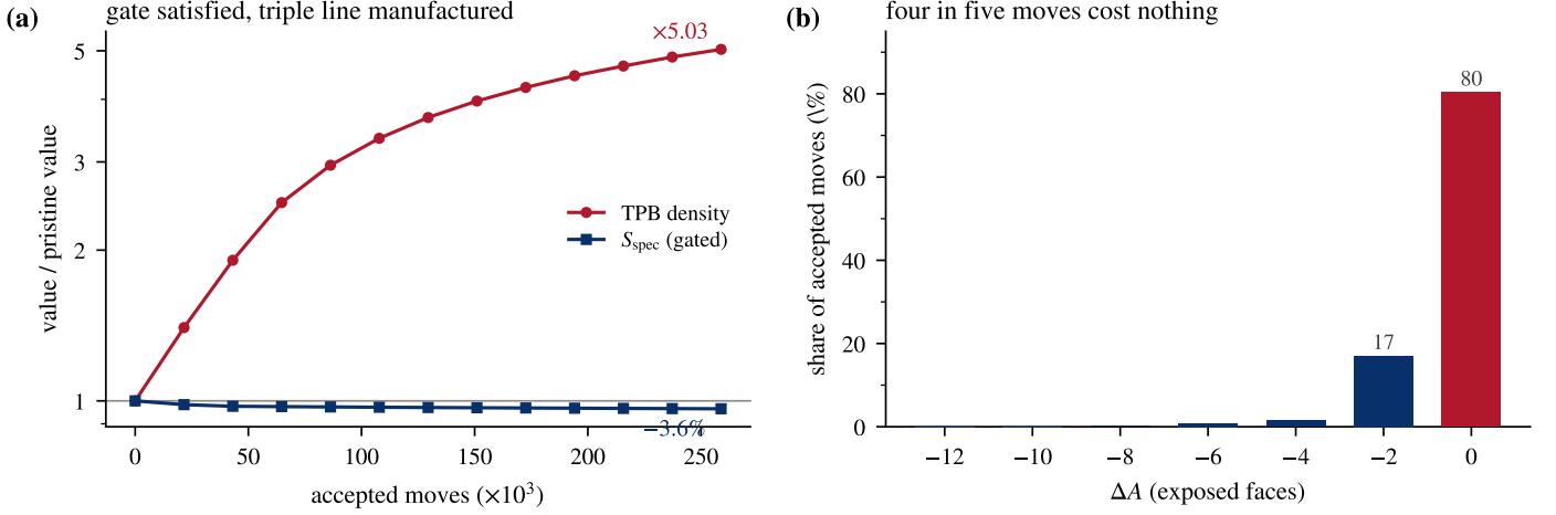
Figure 7: The validity criterion is satisfied while the quantity of interest is destroyed. Fine anode, 67 million voxels, sequential area-decreasing swap, volume conserved exactly. (a) Both quantities are divided by their pristine values so that they share one axis: specific surface area, the gated quantity, falls 3.6 %, while triple-phase-boundary density rises by a factor of 5.03. (b) Why the gate does not object. Accepted moves by their cost in exposed faces; four in five carry \Delta A = 0 exactly and are unpriced by the criterion. Data: o7_trajectory.csv , o7_da_histogram.csv .
