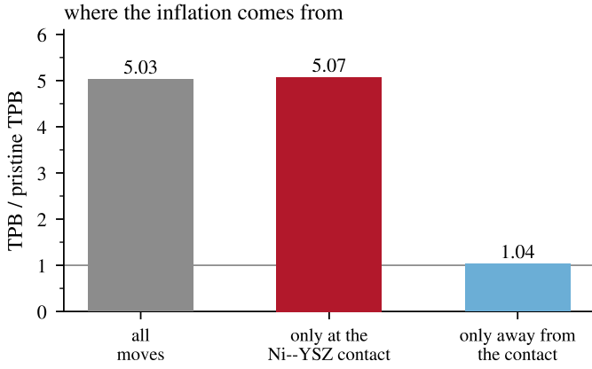
Figure 8: Where the triple-line inflation comes from, by re-applying the two groups of moves separately to the pristine structure. Moves that touch the nickel–zirconia contact reproduce the whole artifact on their own; every other move, 97 % of the added material, changes TPB by four percent. Data: o7_counterfactual.csv .
