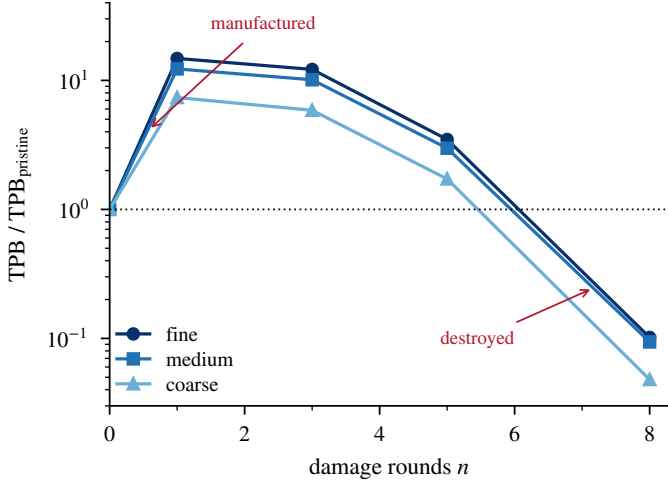
Figure 4: TPB density relative to pristine under surface erosion on real regions of interest. Stochastic single-voxel removal pits the nickel surface, and every new nickel/pore facet touching zirconia creates triple line. Any TPB conclusion drawn before the peak reports discretisation, not the electrode. Data: c1real_rni_gate.csv .
