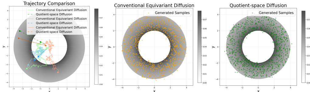
Figure 1: A conceptual illustration highlighting characteristics of the quotient-space diffusion model for a distribution (shown in gray scale) on \mathbb{R}^2 with \text{SO}(2) ( i.e. , rotational) symmetry. (Left) SDE sampling trajectories. Same color indicates the same starting point (round dot). The quotient-space diffusion moves only radially along rays emanating from the origin, representing the quotient space \mathbb{R}^2/\text{SO}(2) which traverses across equivalence classes (origin-centered concentric circles) without moving within an equivalence class (angular movement). The conventional diffusion model moves over the whole \mathbb{R}^2 space, leading to jagged curves requiring subtler simulation. (Middle) Samples generated by the conventional equivariant diffusion model and (Right) by the quotient-space diffusion model. Both recover the same target distribution. The quotient-space diffusion also reduces learning difficulty (Eq. (11)) by allowing arbitrary model output in intra-equivalence-class movement (angular movement).
