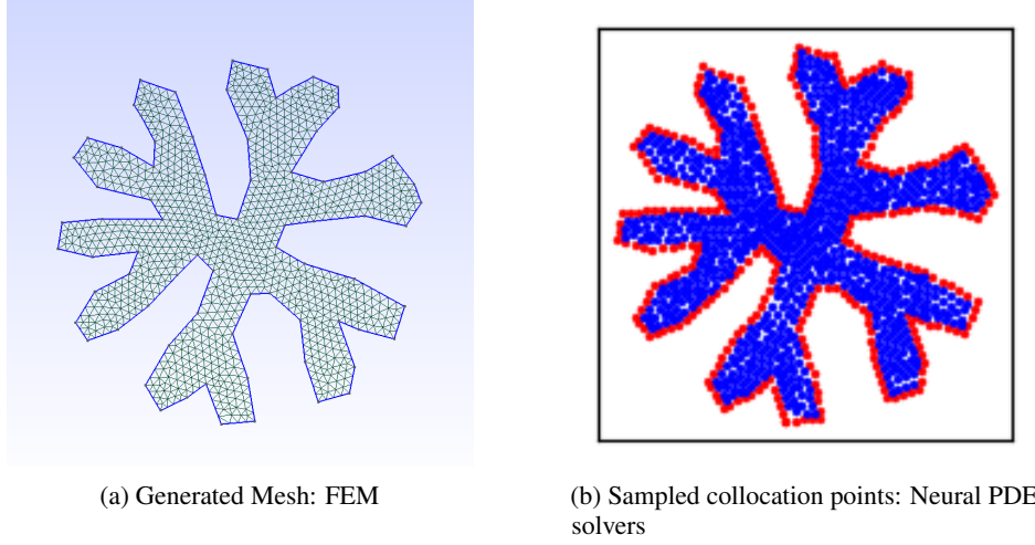
Figure 24: Advantages of mesh-free methods: (a) For mesh-based methods, a complicated mesh must be constructed, whereas (b) for neural PDE solvers, one can easily sample arbitrary points in the interior (blue) and on the boundary (red) of the domain and work directly with point clouds.
