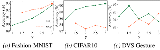
Figure 9. Comparisons of weight decay methods with different \gamma values for the temporal weighting decoder method on three datasets. The highest accuracy on each dataset is marked by ★.
