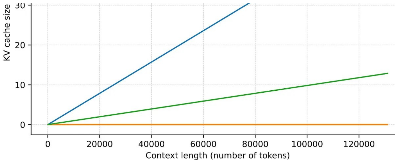
Figure 25: The practical motivation behind the hybrids is shown here in the memory curve. Hybrid stacks with Gated DeltaNet grow much more slowly with context length than ordinary full attention (Original source LLMs-from-scratch DeltaNet materials ).
