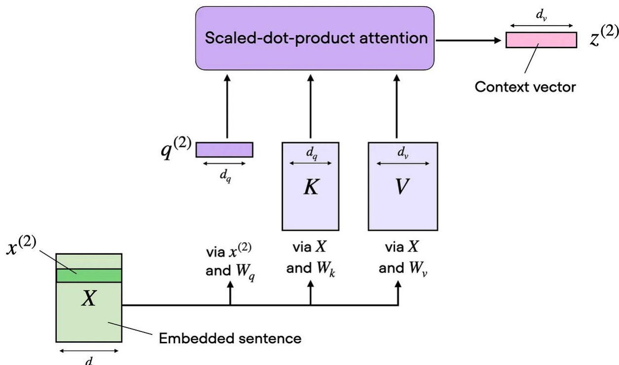
Figure 8: One attention head is already a complete mechanism. One set of learned projections produces one attention matrix and one context-aware output stream (Original source Understanding and Coding Self-Attention ).
