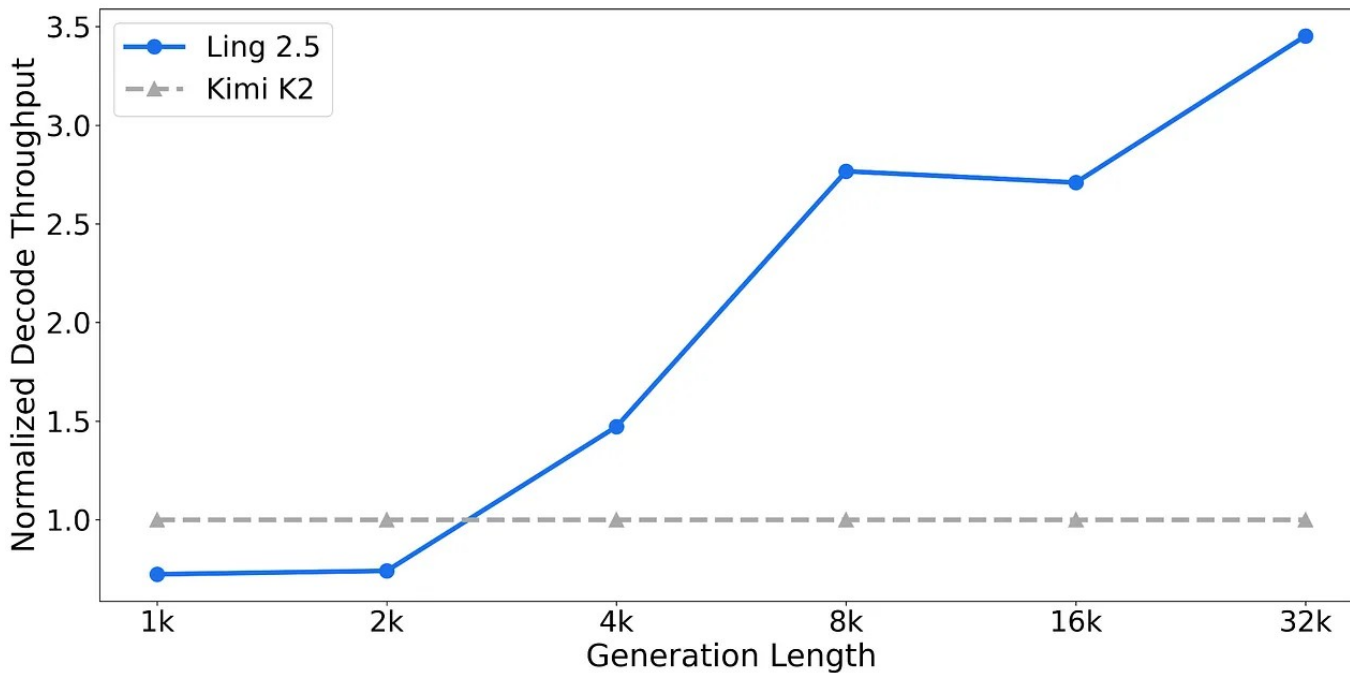
Figure 29: Ling 2.5 was presented as a strong efficiency upgrade, with much higher 32k-token throughput than Kimi K2 at the same 1-trillion-parameter scale (Original source Ling 2.5 model hub page ).
