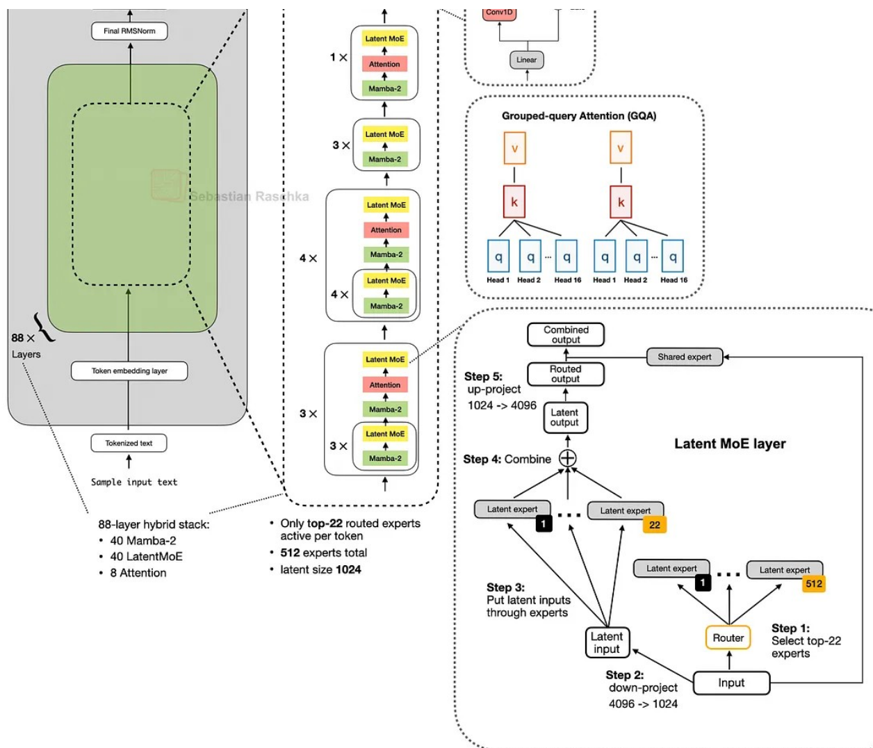
Figure 31: Nemotron 3 Super keeps the Mamba-2 hybrid attention pattern while adding latent MoE and shared-weight MTP on top (Original source The Big LLM Architecture Comparison ).
