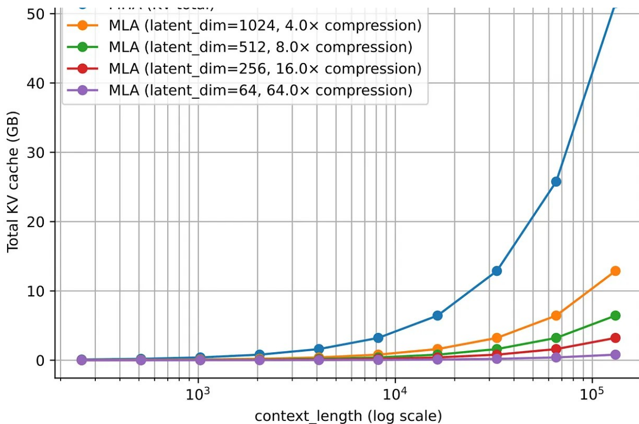
Figure 14: Once context length grows, the savings from caching a latent representation instead of full K/V tensors become very visible (Original source: LLMs-from-scratch MLA section).
