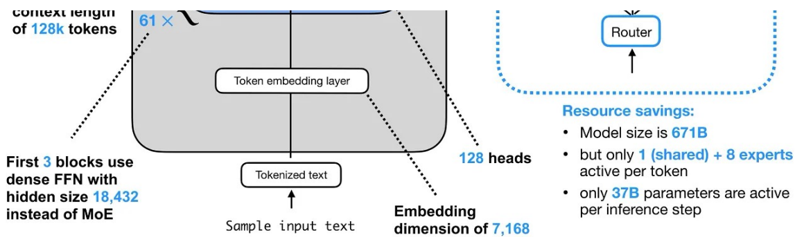
Figure 20: DeepSeek V3.2 is the obvious reference point, because this is the model family most closely associated with the sparse-attention idea.
