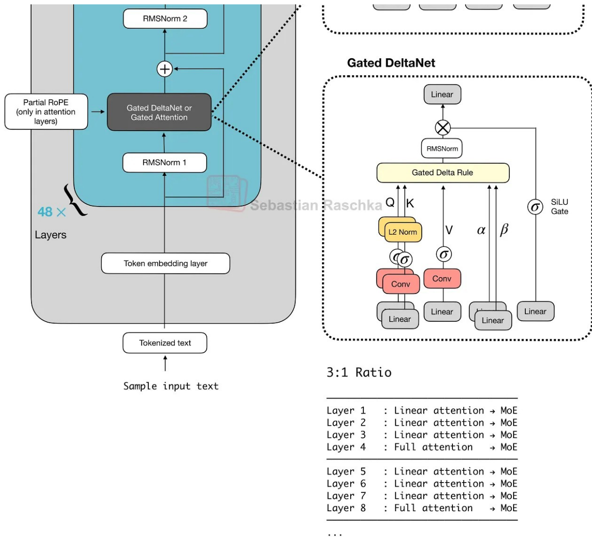
Figure 23: In Qwen3-Next and Qwen3.5, gated attention appears as the full-attention layer that periodically breaks up runs of Gated DeltaNet blocks.
