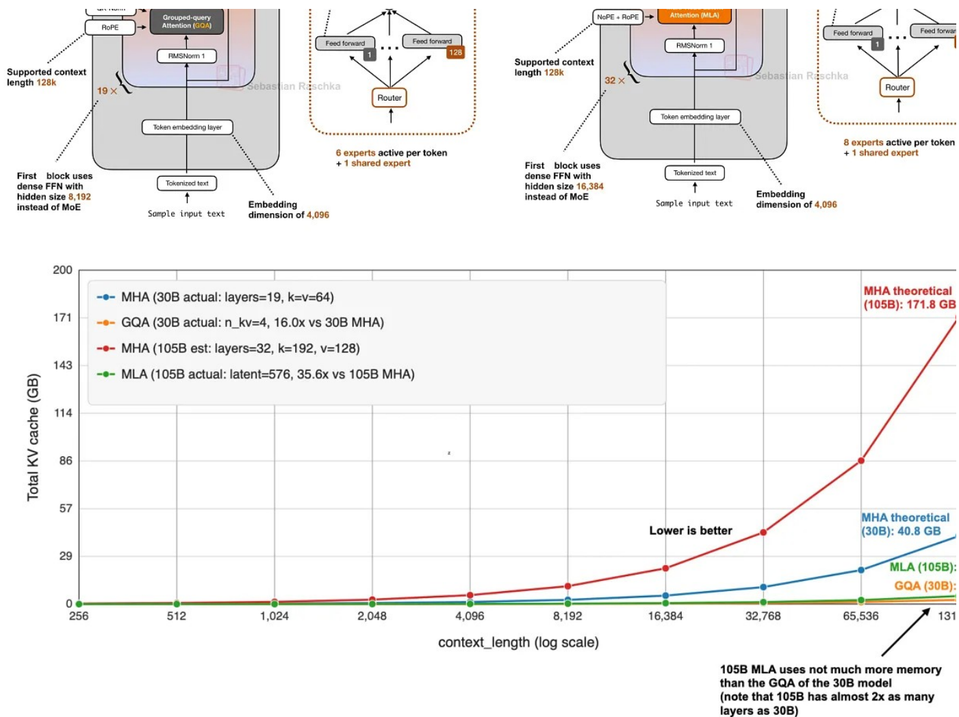
Figure 16: GQA and MLA are solving the same bottleneck from different directions. The tradeoff is simplicity versus better modeling performance for larger models.
