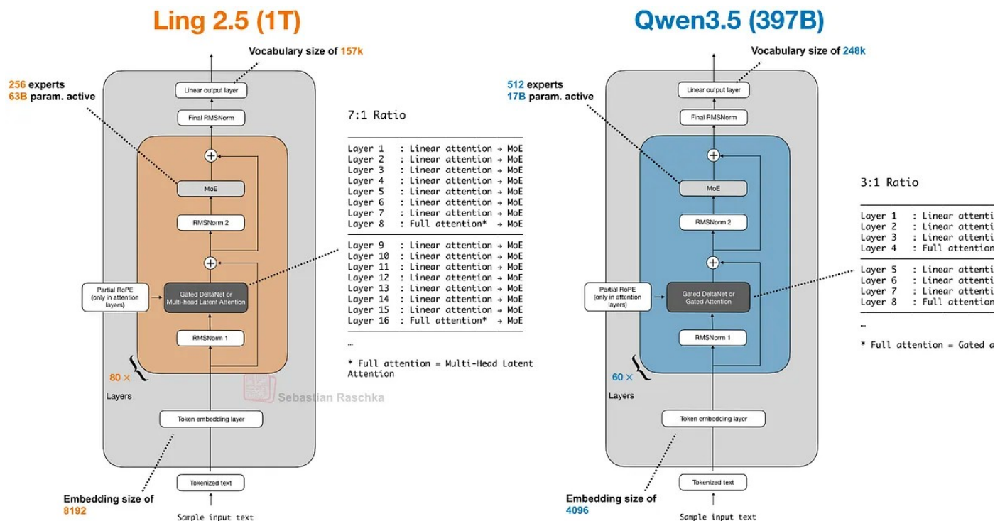
Figure 28: Ling 2.5 and Qwen3.5 are both linear-attention hybrids, even though Ling swaps in Lightning Attention and MLA instead of the Qwen recipe (Original source A
