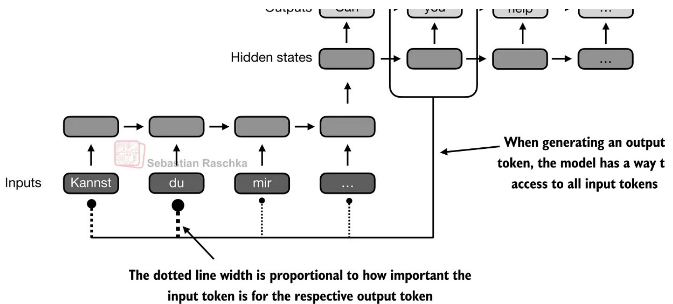
Figure 5: Attention breaks the RNN bottleneck by letting the current output position revisit the full input sequence instead of relying on one compressed state alone (Original source LLMs-from-scratch ).
