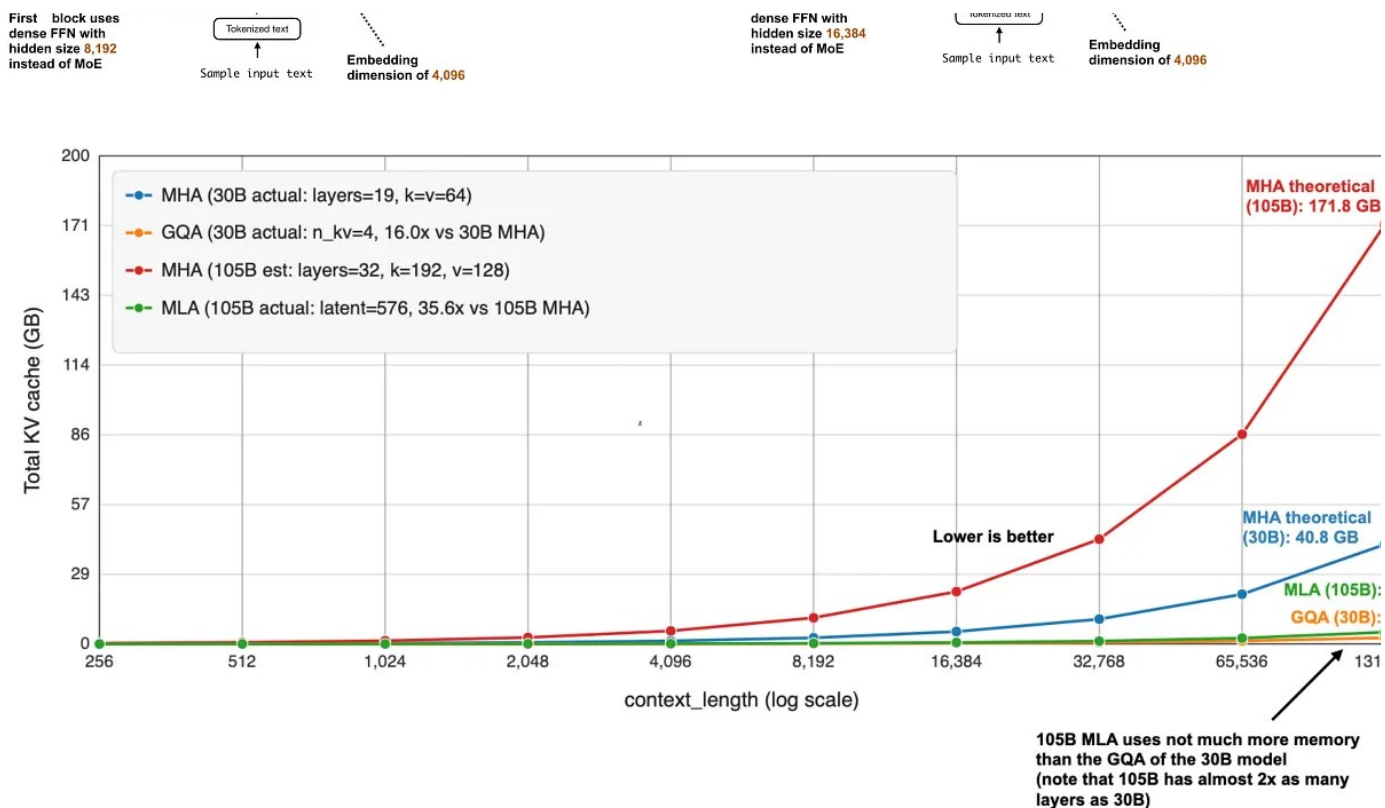
Figure 12: Total KV cache sizes for 105B Sarvam (using MLA) versus 30B Sarvam (using GQA), versus using plain MHA.
