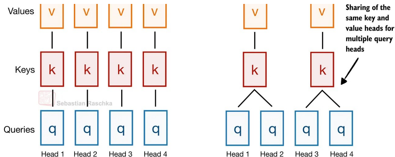
Figure 10: GQA keeps the same overall attention pattern as MHA, but collapses the number of key-value heads by sharing them across multiple query heads (Original source: The Big LLM Architecture Comparison ).
