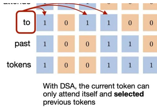
Figure 19: Similar to sliding-window attention, DeepSeek Sparse Attention also restricts each token to a subset of prior tokens, but does not do so with a fixed local window (Original source: From DeepSeek V3 to V3.2: Architecture, Sparse Attention, and RL Updates ).
