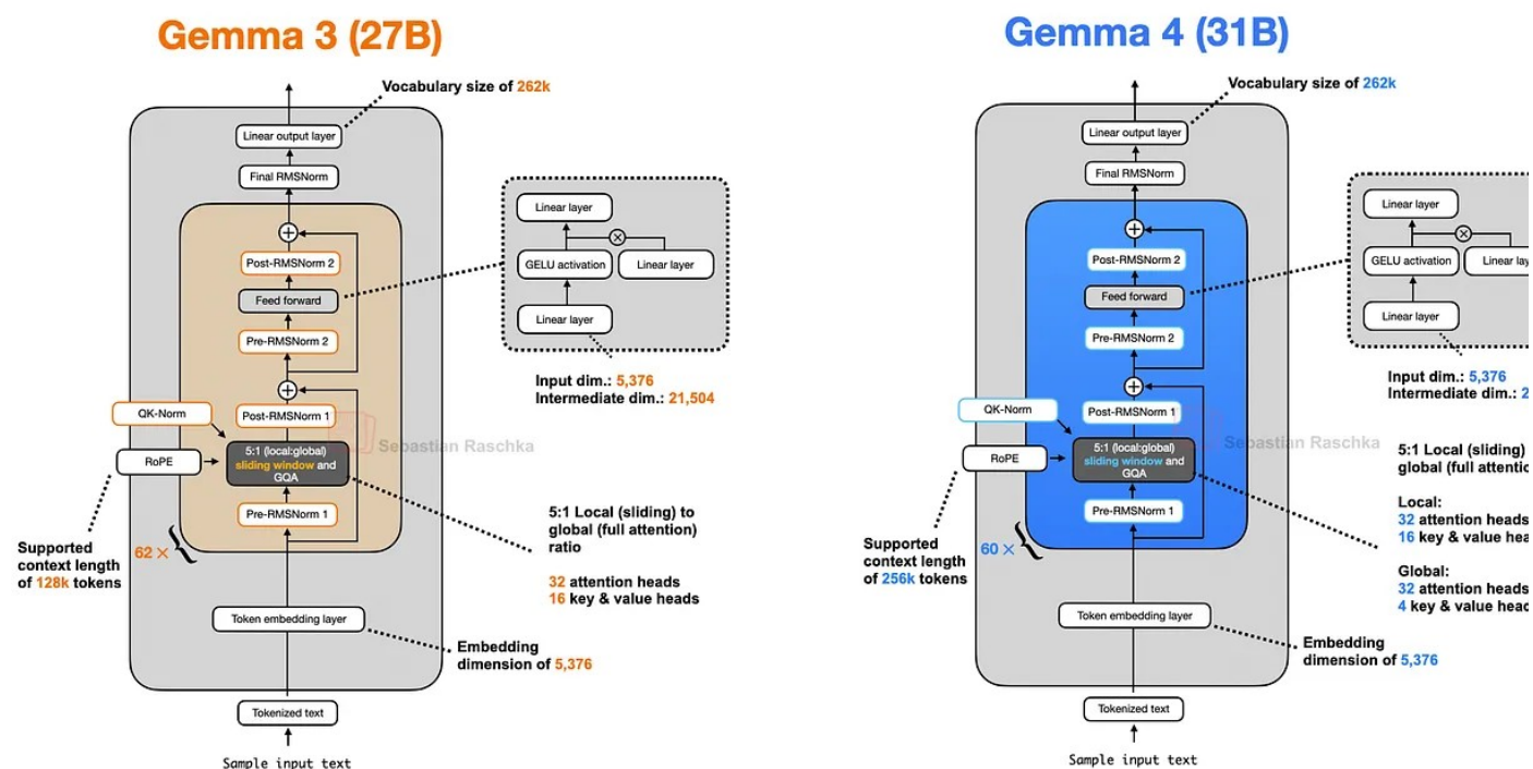
Figure 58: Gemma 3 (27B) and Gemma 4 (31B) side by side.
