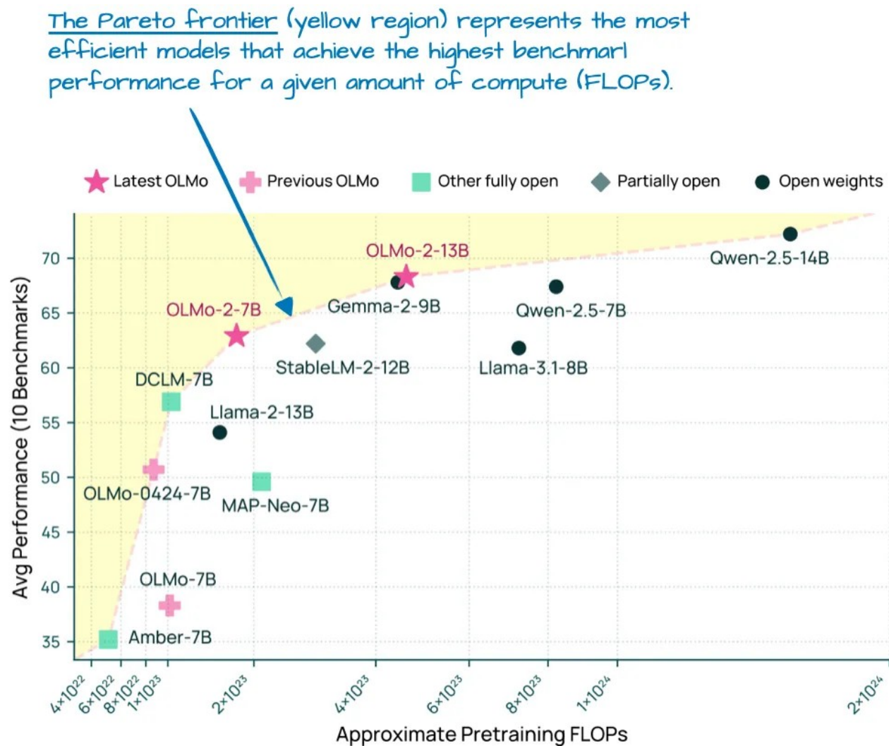
Figure 7: Modeling benchmark performance (higher is better) vs pre-training cost (FLOPs; lower is better) for different LLMs. This is an annotated figure from the OLMo 2 paper, https://arxiv.org/abs/2501.00656
