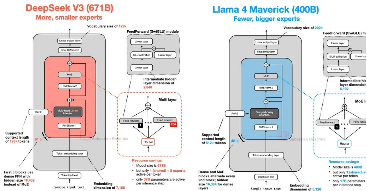
Figure 17: An architecture comparison between DeepSeek V3 (671-billion parameters) and Llama 4 Maverick (400-billion parameters).
