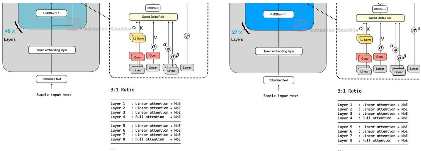
Figure 42: Qwen3-Next and Kimi Linear side by side.
