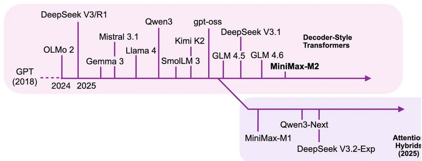
Figure 38: A timeline of the main LLMs covered in this article, next to some of the attention-hybrid models that constitute more efficient alternatives, trading off some modeling performance with improved efficiency.
