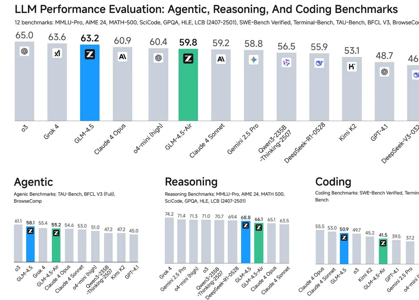
Figure 33: GLM-4.5 benchmark from the official GitHub repository at https://github.com/zai-org/GLM-4.5
