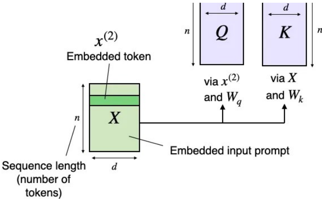
Figure 40: Illustration of the quadratic cost in attention due to sequence length n .
