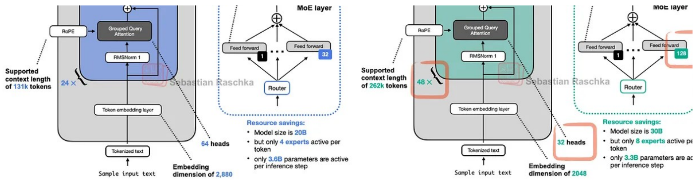
Figure 27: Architecture comparison between gpt-oss and Qwen3
