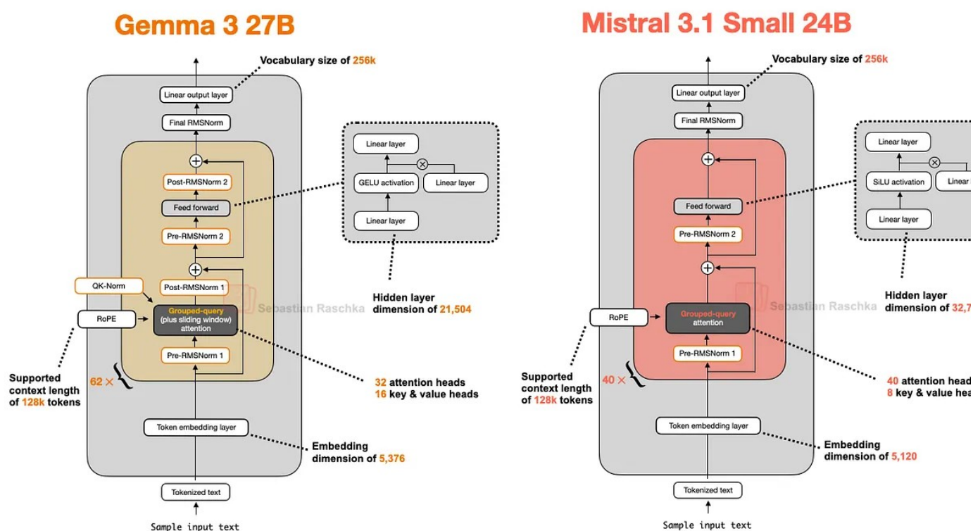
Figure 16: An architecture comparison between Gemma 3 27B and Mistral 3.1 Small 24B.
