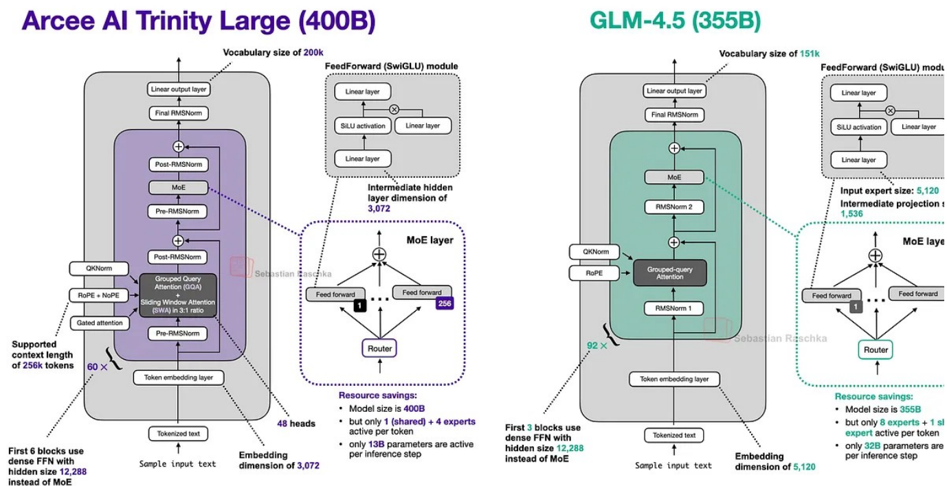
Figure 54: Arcee AI Trinity Large next to GLM 4.5 of a relatively similar size (400B vs 355B).
