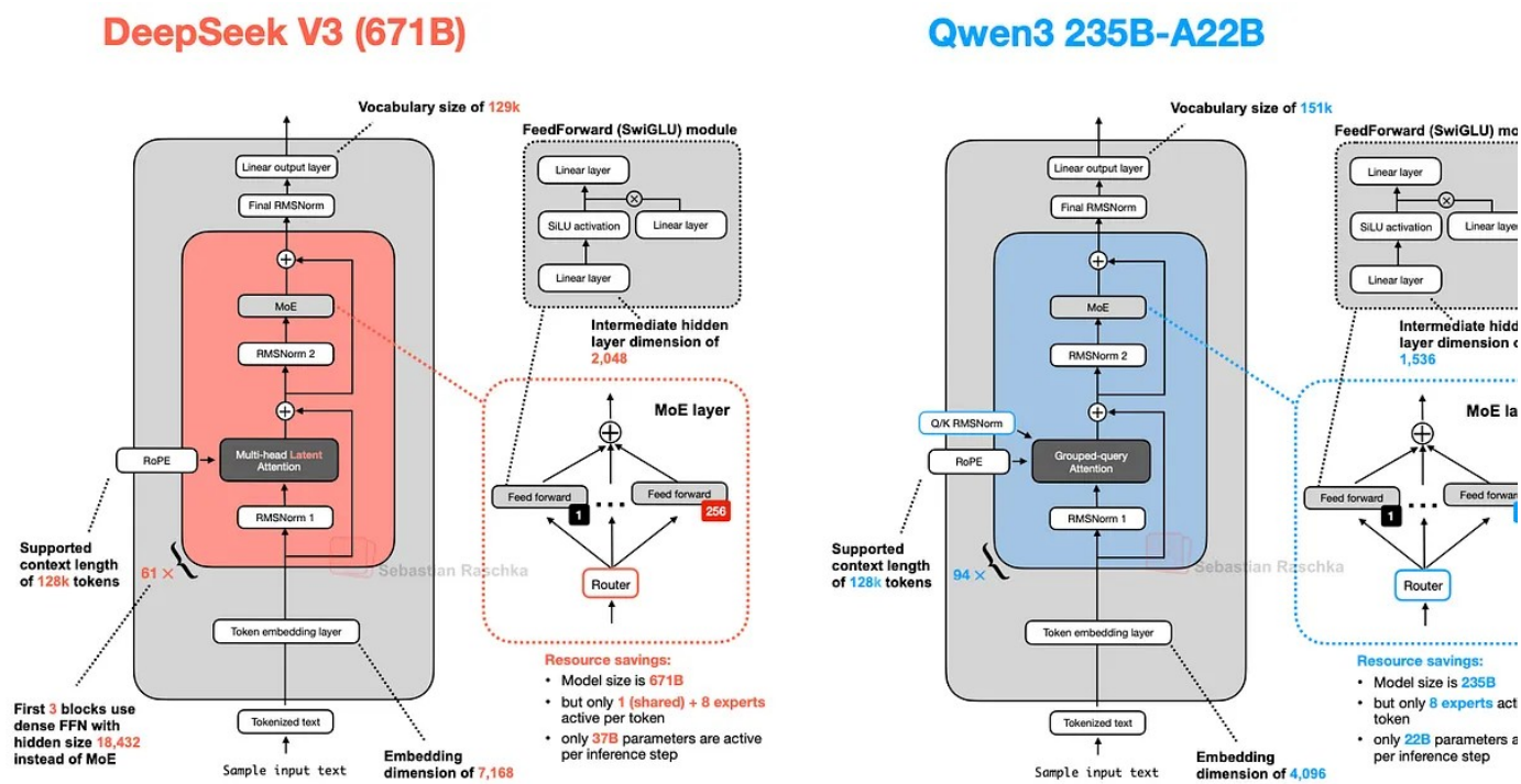
Figure 19: An architecture comparison between DeepSeek V3 and Qwen3 235B-A22B.
