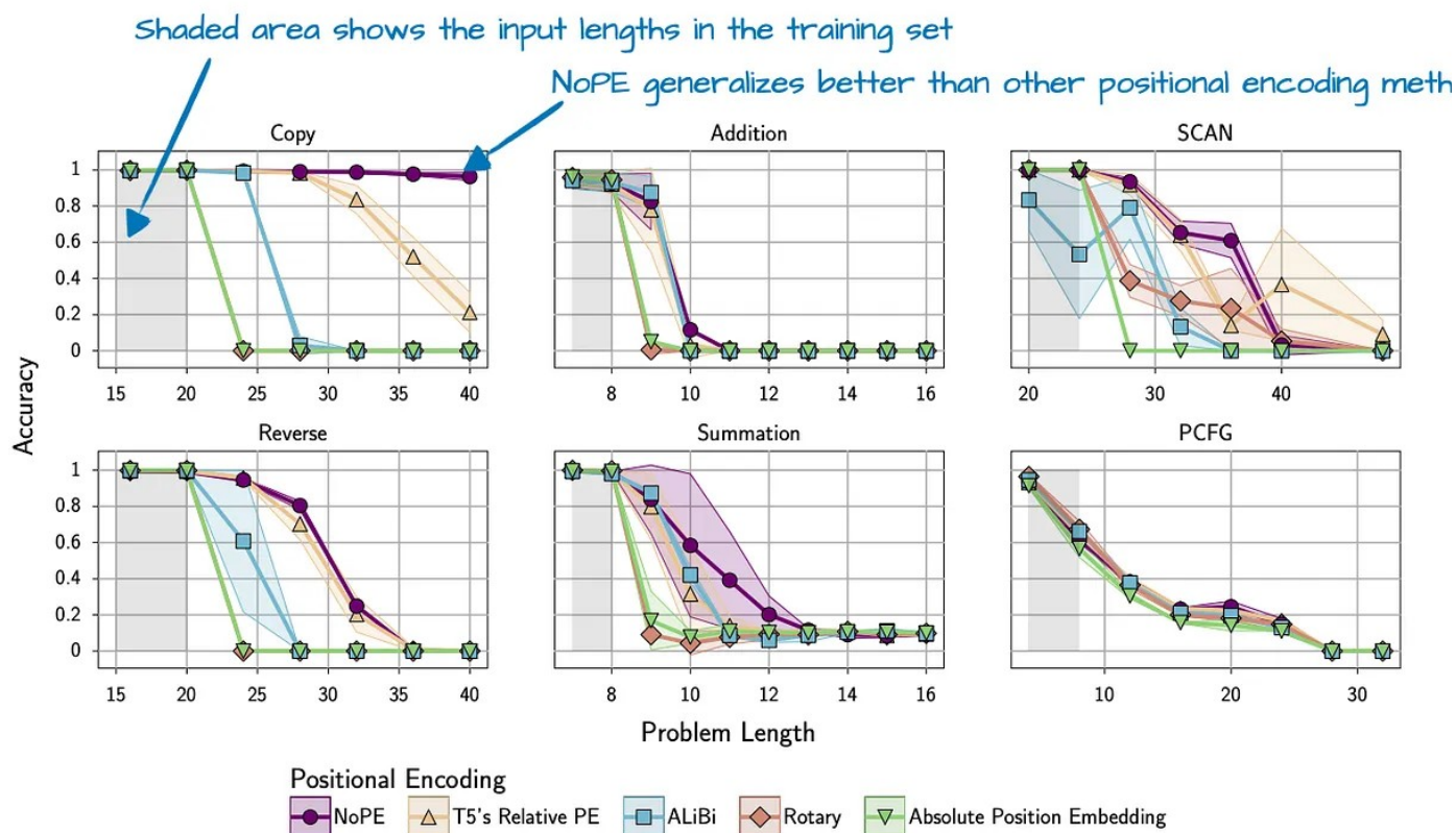
Figure 23: An annotated figure from the NoPE paper ( https://arxiv.org/abs/2305.19466 ) showing better length generalization with NoPE.
