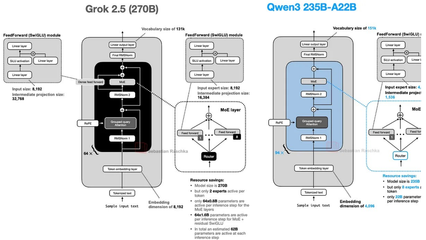
Figure 32: Grok 2.5 next to a Qwen3 model of comparable size
