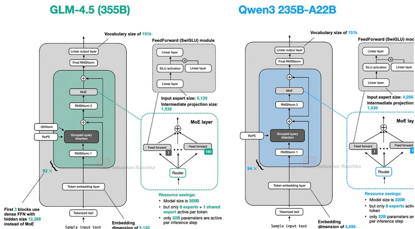
Figure 34: GLM-4.5 next to a similarly-sized Qwen3 model.
