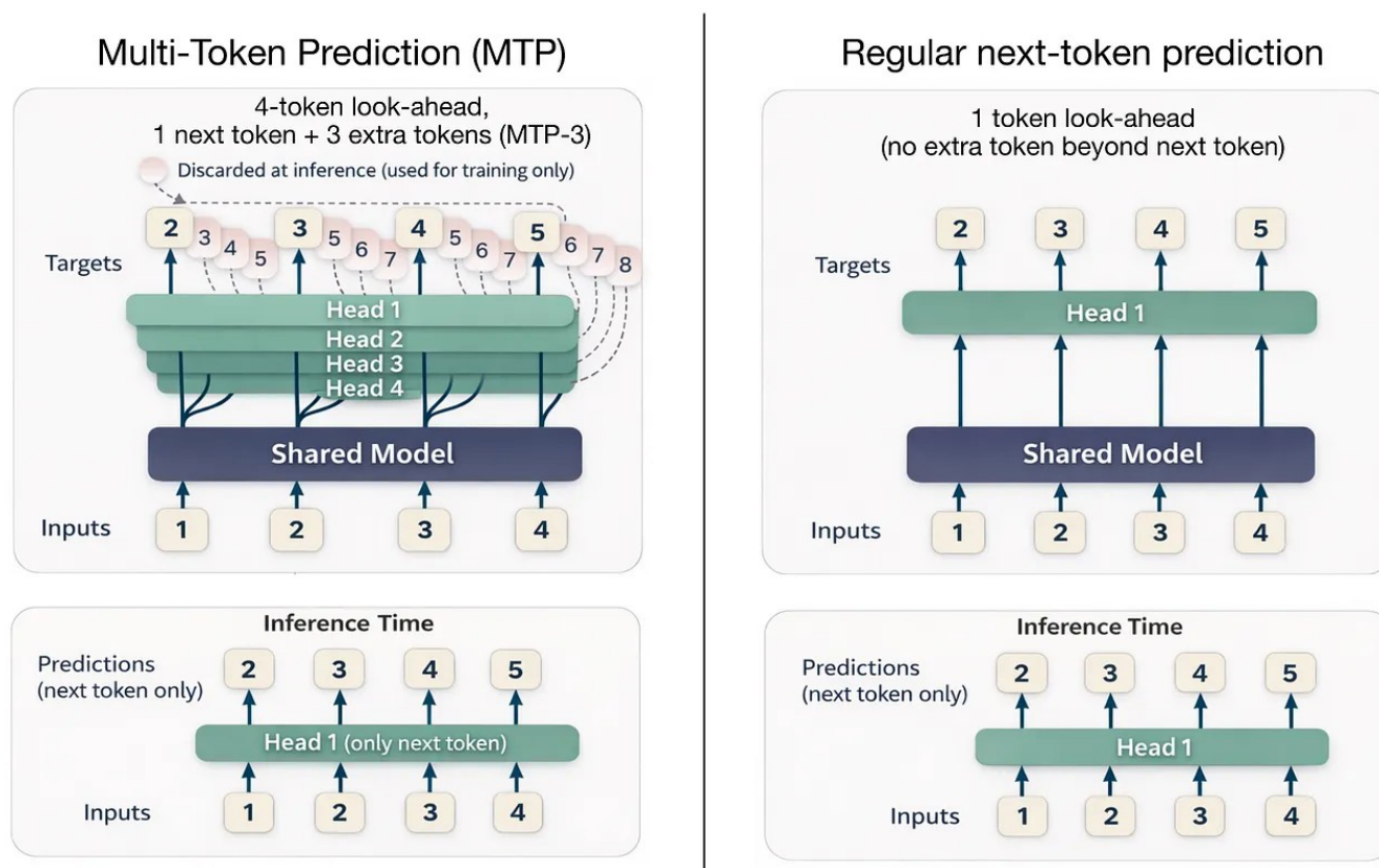
Figure 51.2: Multi-Token Prediction versus regular next token prediction. (Left subfigure inspired by the MTP paper .) Originally, MTP was only used during training, not inference; hence, the inference time steps (bottom) show a single next-token prediction.
