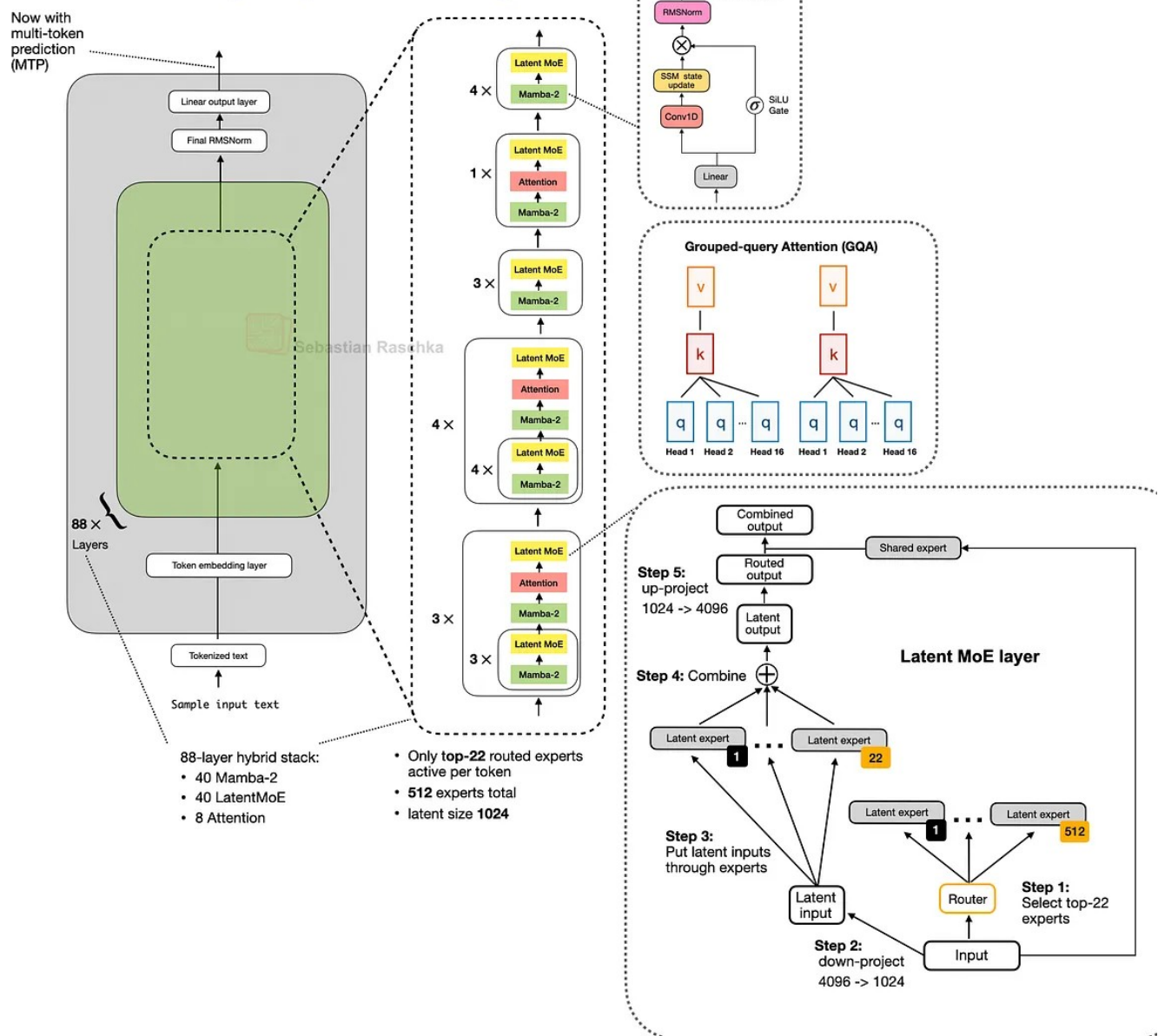
Figure 51.3: Nemotron 3 Super 120B-A12B with latent MoE layers, multi-token prediction, and the Mamba-2 hybrid attention approach.
