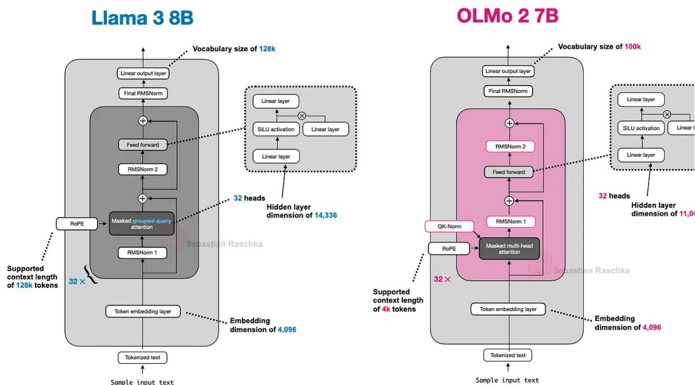
Figure 10: An architecture comparison between Llama 3 and OLMo 2.
