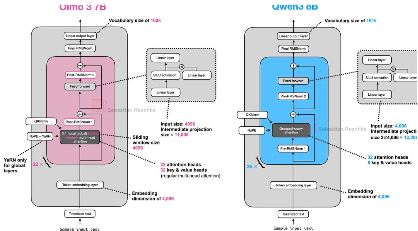
Figure 44: Olmo 3 7B and Qwen3 8B side by side.
