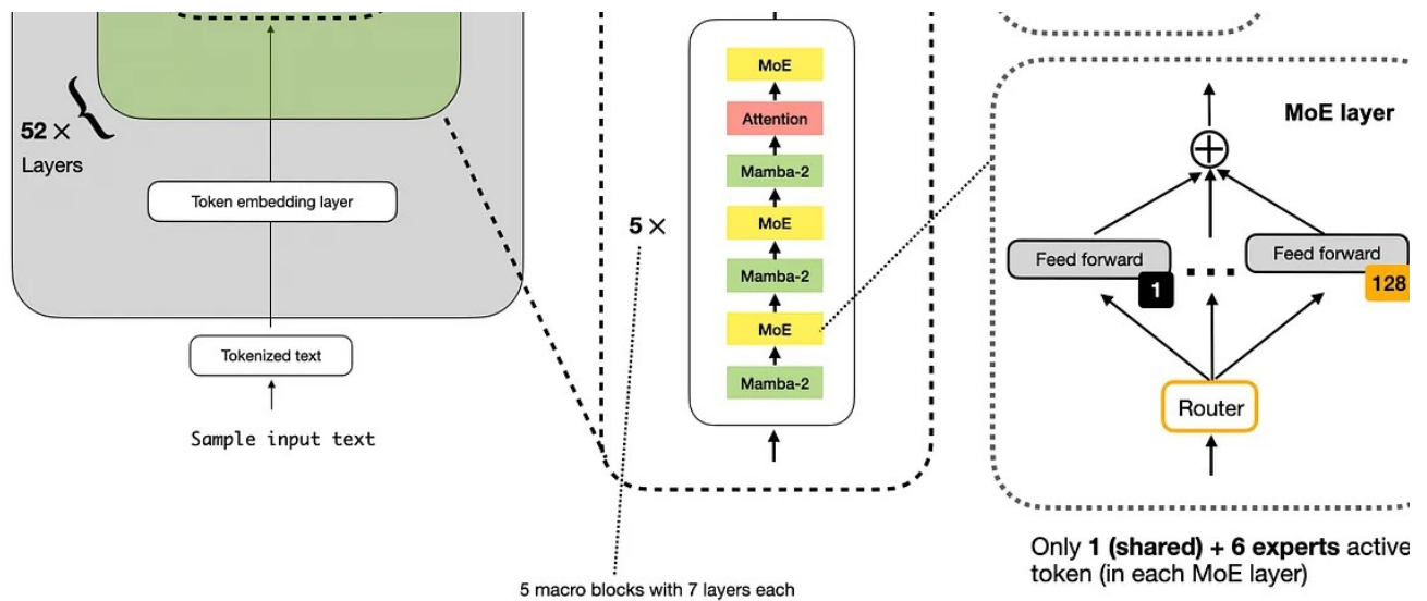
Figure 51.1: Outline of the Nemotron 3 Nano model, which is a Transformer-Mamba hybrid.
