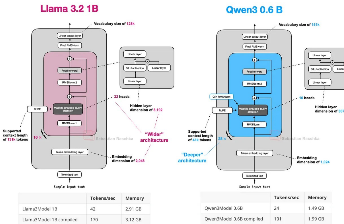
Figure 18: An architecture comparison between Qwen3 0.6B and Llama 3 1B; notice that Qwen3 is a deeper architecture with more layers, whereas Llama 3 is a wider architecture with more attention heads.
