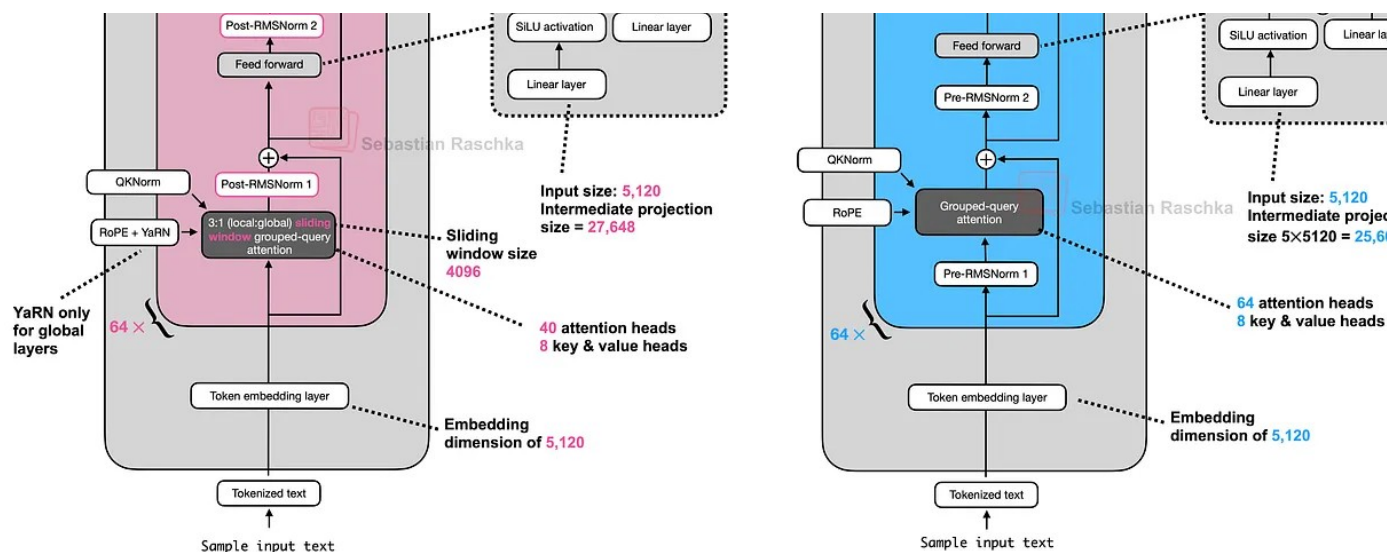
Figure 45: Olmo 3 32B and Qwen3 32B side by side.
