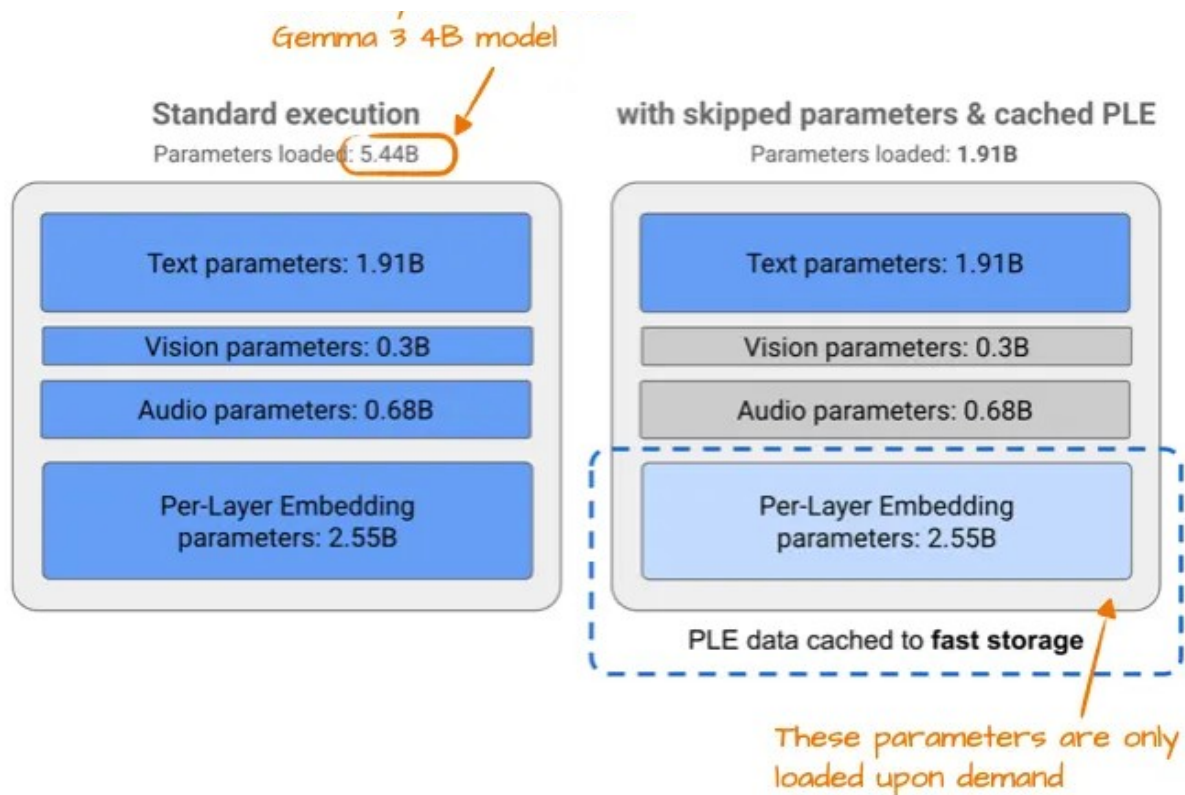
Figure 15: An annotated figure from Google's Gemma 3n blog ( https://developers.googleblog.com/en/introducing-gemma-3n/ ) illustrating the PLE memory savings.
