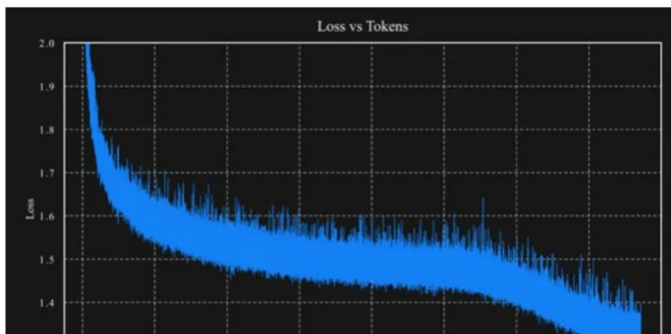
Kimi K2 training loss curve
