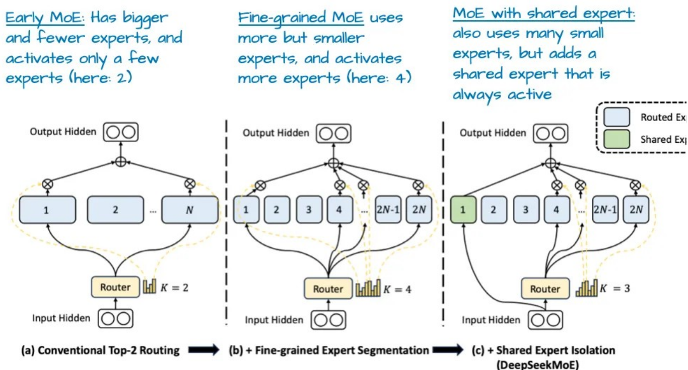
Figure 6: An annotated figure from "DeepSeekMoE: Towards Ultimate Expert Specialization in Mixture-of-Experts Language Models", https://arxiv.org/abs/2401.06066
