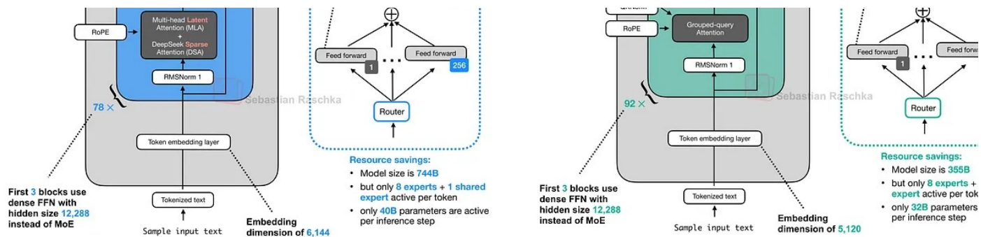
Figure 56: Architecture of GLM-5 and GLM-4.5 side by side.
