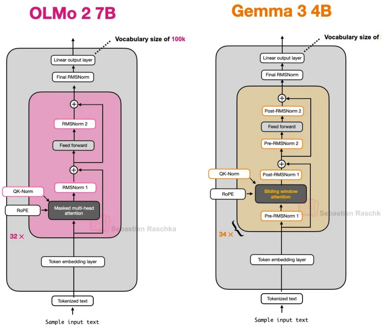
Figure 14: An architecture comparison between OLMo2 and Gemma 3; note the additional normalization layers in Gemma 3.
