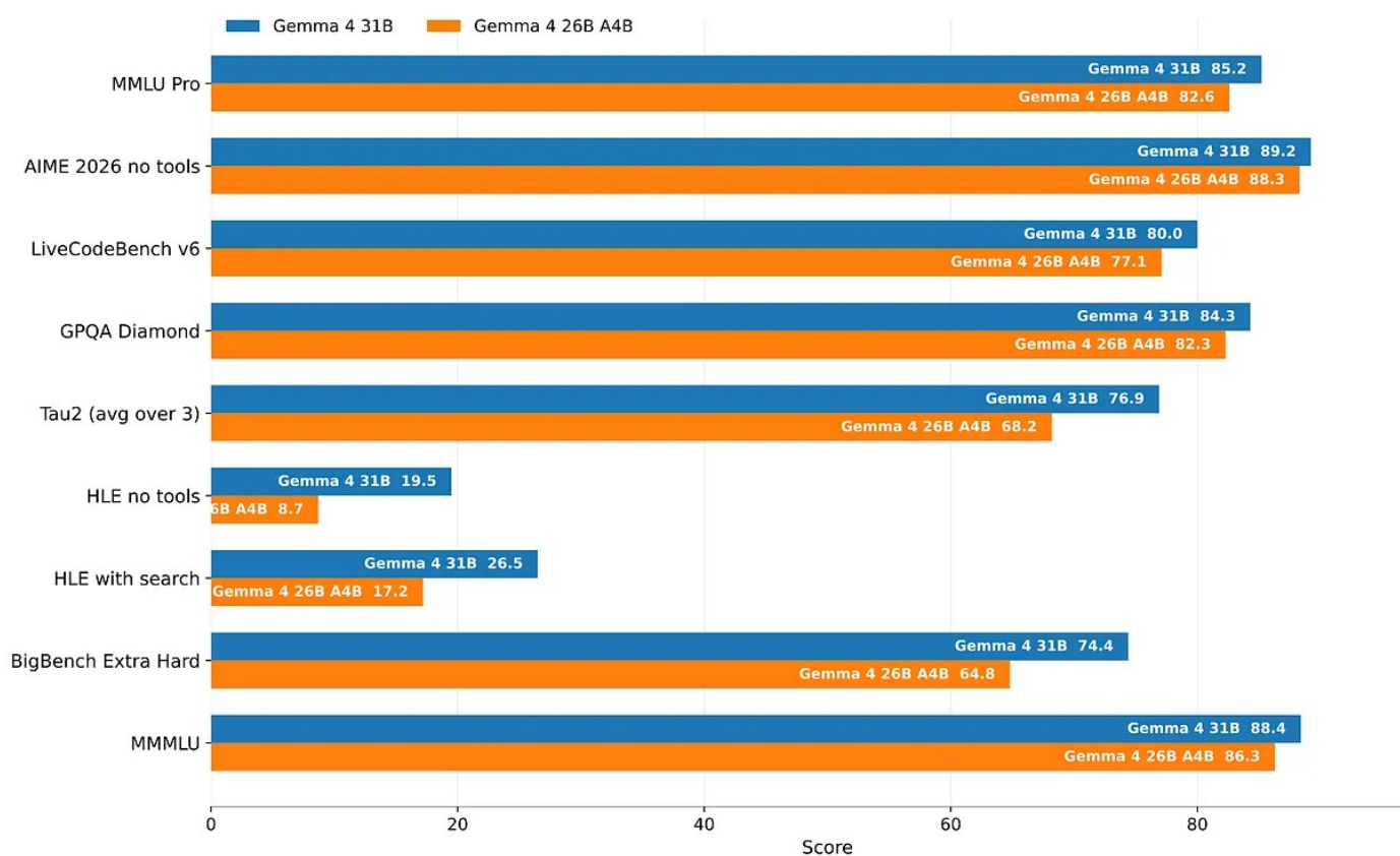
Figure 61: Gemma 4 MoE (26B-A4B) is only slightly worse than Gemma 4 (31) dense.
