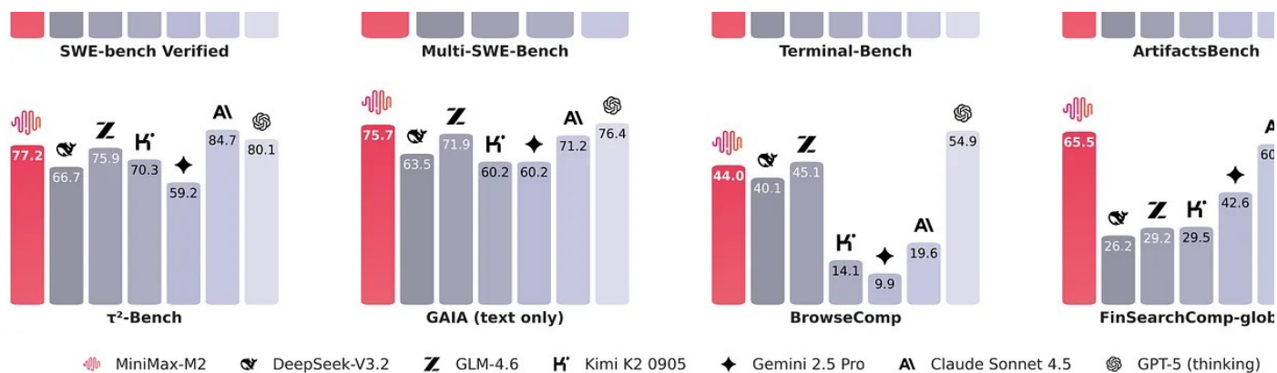
Figure 37: MiniMax-M2 benchmark performance compared to other popular open-weight and proprietary LLMs. Image from the official model hub release readme file.
