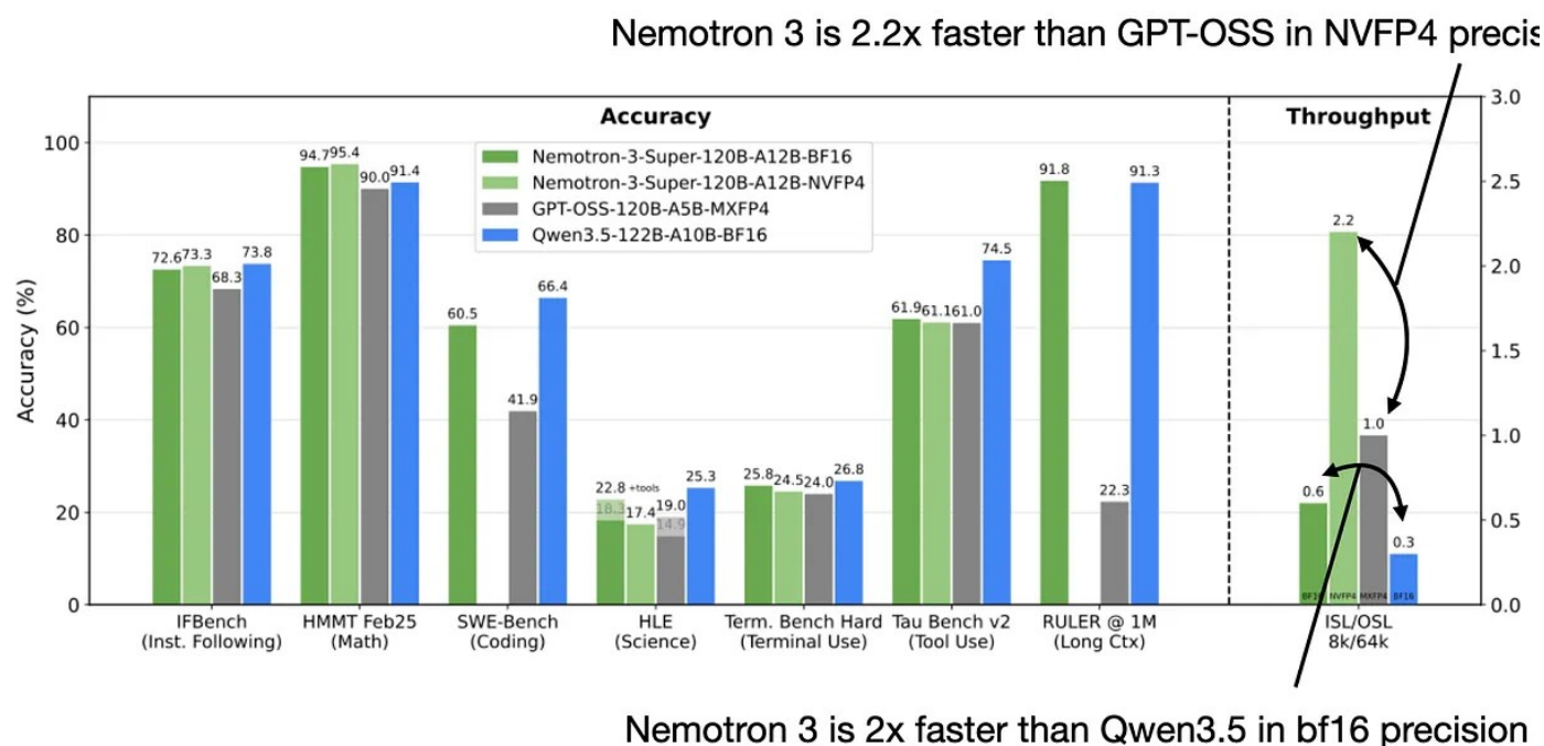
Figure 51.4: Nemotron 3 Super benchmark comparison from the Hugging Face Hub page.
