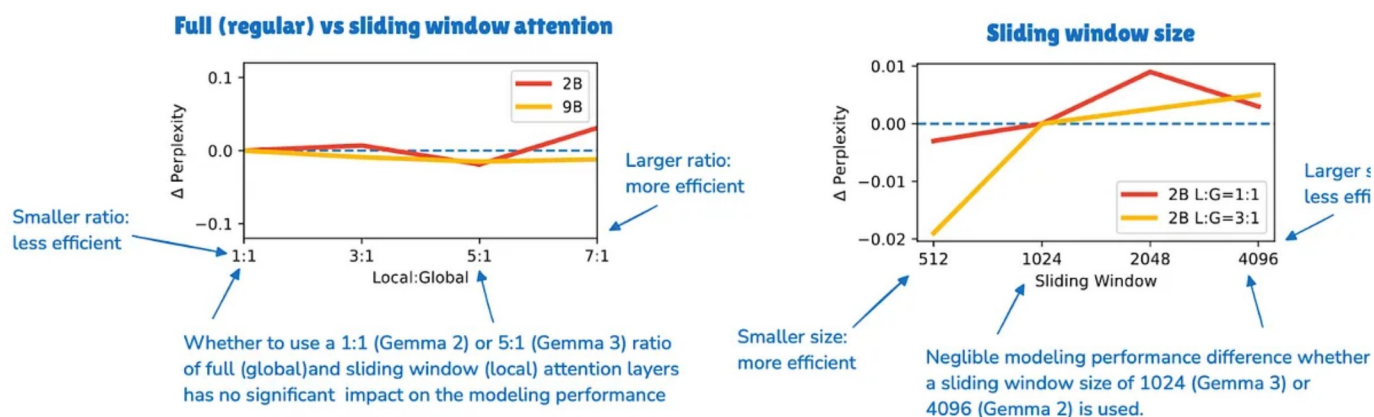
Figure 13: An annotated figure from Gemma 3 paper ( https://arxiv.org/abs/2503.19786 ) showing that sliding window attention has little to no impact on the LLM-generated output perplexity.
