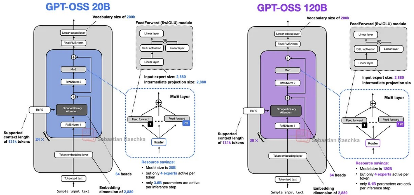
Figure 26: Architecture overview of the two gpt-oss models.
