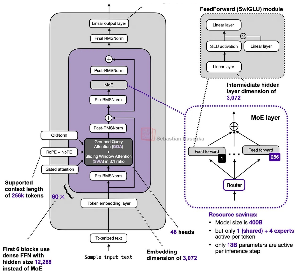
Figure 53: Overview of the Trinity Large architecture (based on the model hub config file ).
