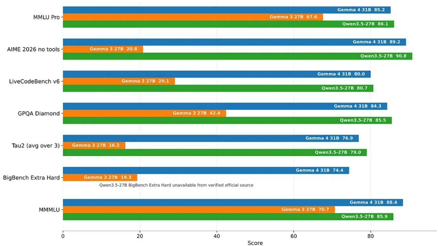
Figure 59: Gemma 3 versus Gemma 4 versus Qwen3.5 (the numbers are taken from the Gemma 4 and Qwen3.5 model hub pages).
