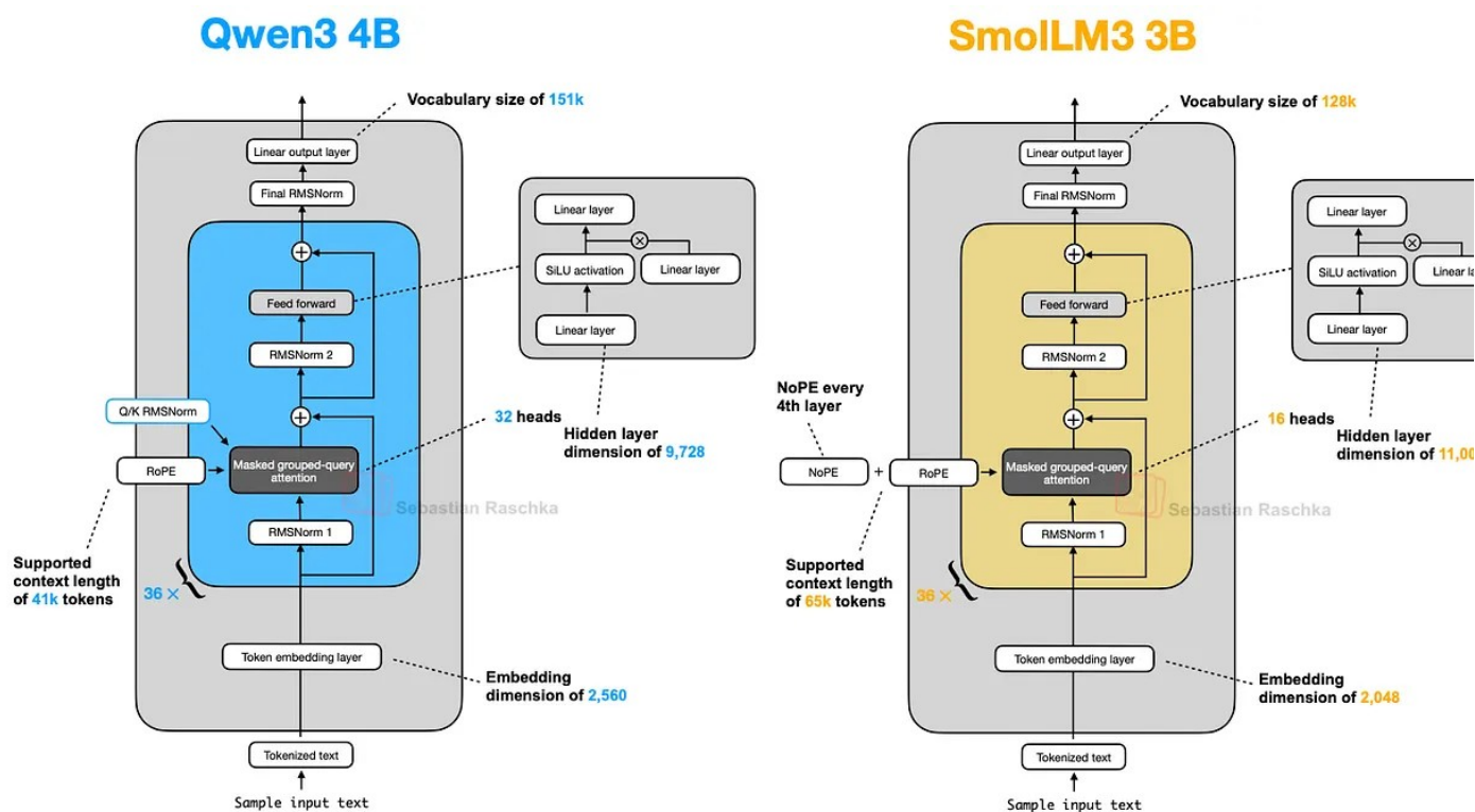
Figure 21: A side-by-side architecture comparison between Qwen3 4B and SmolLM3 3B.
