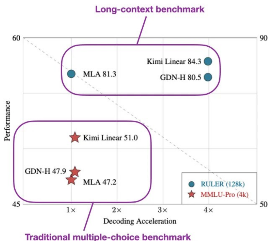
Figure 43: Annotated figure from the Kimi Linear paper showing that Kimi Linear is as fast as GatedDeltaNet, and much faster than an architecture with multi-head
