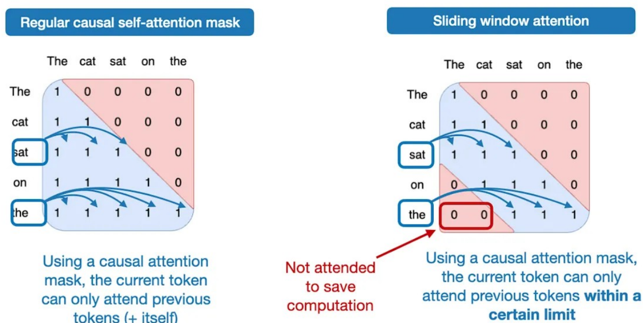
Figure 12: A comparison between regular attention (left) and sliding window attention (right).
