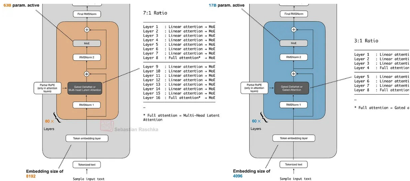
Figure 32: Ling 2.5 compared to Qwen3.5; both architectures are linear attention hybrids.
