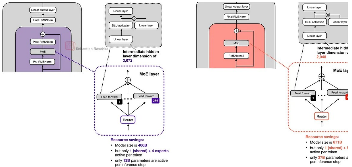
Figure 6: Arcee Trinity and DeepSeek V3/R1 MoE side by side.
