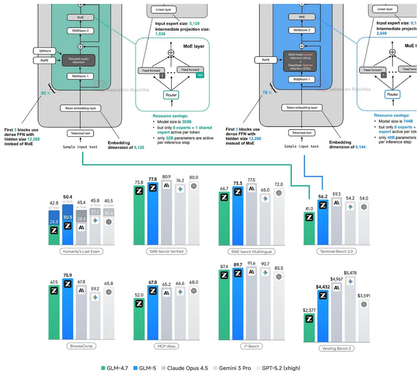
Figure 18: GLM-5 architecture next to its GLM-4.7 predecessor. Benchmarks at the bottom taken from the official GLM-5 technical report .
