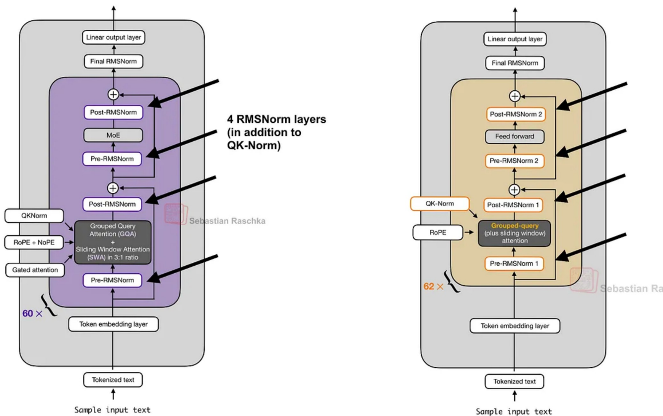
Figure 5: Arcee Trinity and Gemma 3 RMSNorm placement side by side.
