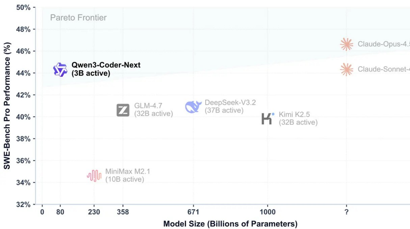
Figure 14: Qwen3-Coder-Next performance on a coding benchmark next to other popular coding models; this figure appeared in the official technical report .
