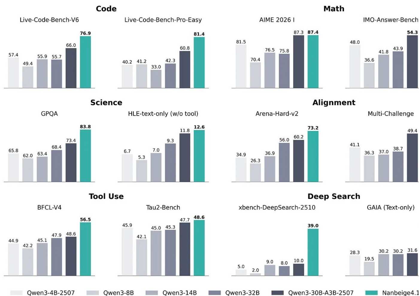
Figure 28: Nanbeige 4.1 3B benchmark comparison with Qwen3 (Source: Nanbeige 4.1 3B model hub page ).
