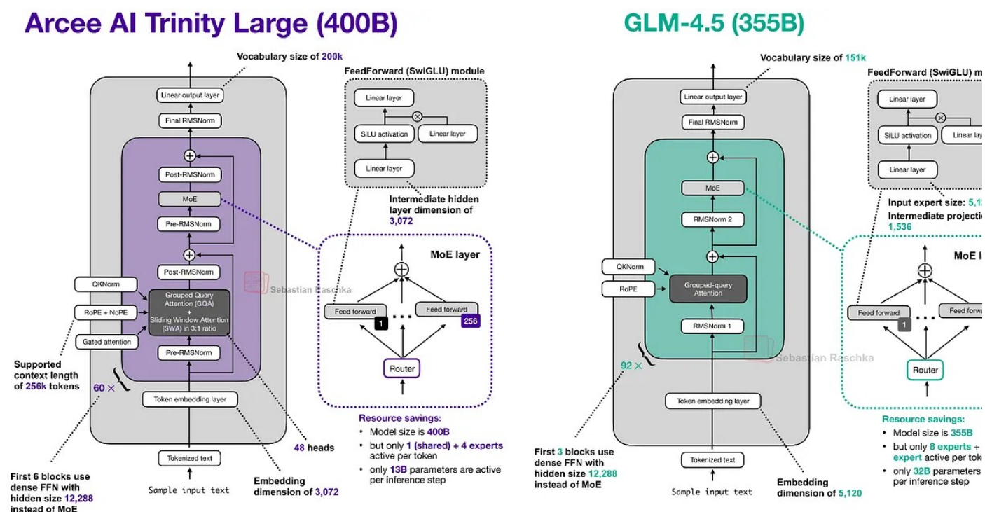
Figure 2: Arcee AI Trinity Large next to GLM-4.5 of a relatively similar size (400B vs
