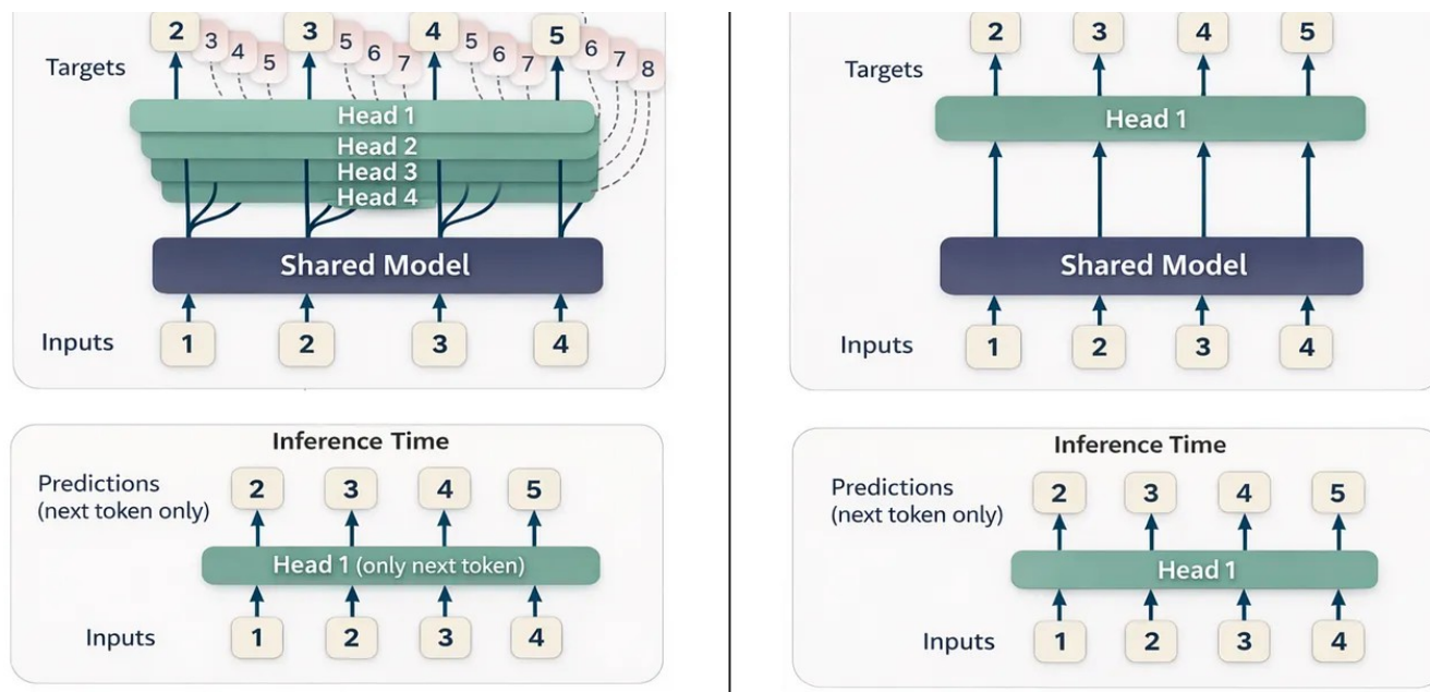
Figure 13: Multi-Token Prediction versus regular next token prediction. (Left subfigure inspired by the MTP paper .) Originally, MTP was only used during training, not inference; hence, the inference time steps (bottom) show a single next-token prediction.
