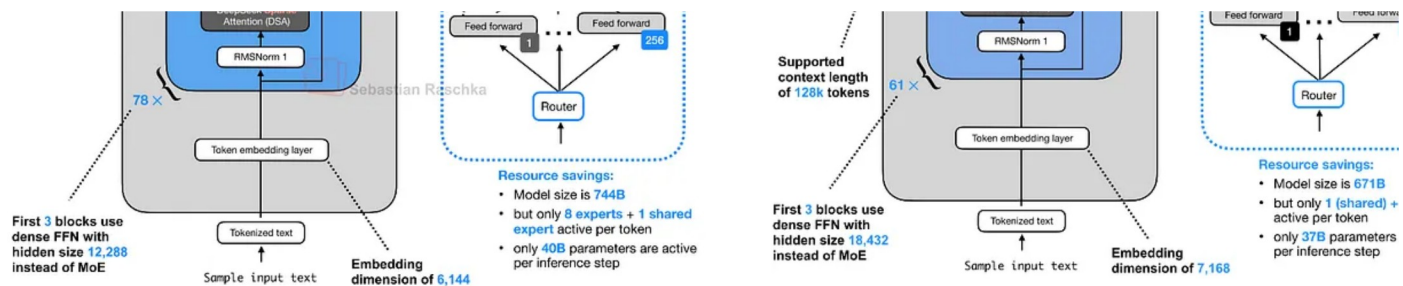
Figure 20: GLM-5 and DeepSeek V3.2 side by side (two similar architectures at a similar size).
