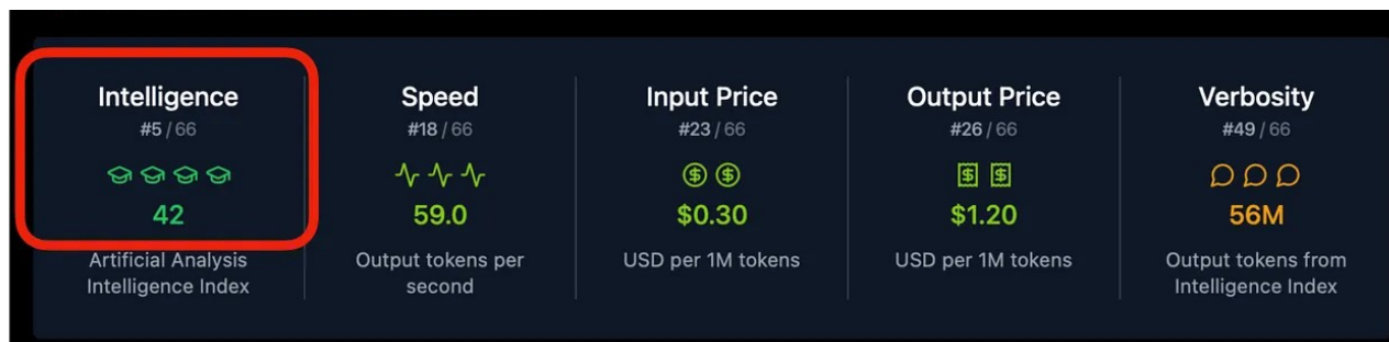
Figure 25: GLM-5 vs MiniMax M2.5 comparison based on the Artificial Intelligence Index (Feb 21, 2026)
