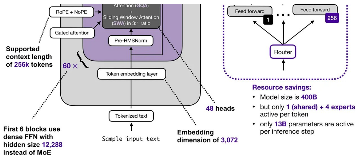
Figure 1: Overview of the Trinity Large architecture (based on the model hub config file ).
