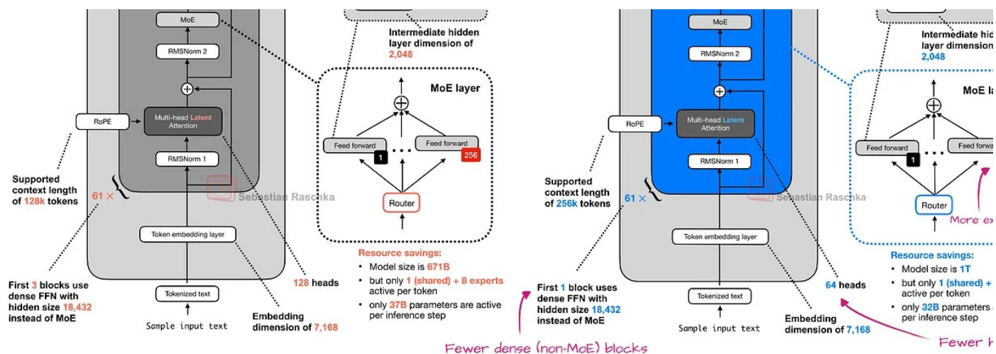
Figure 8: Kimi K2 is a larger version of the DeepSeek V3 architecture.
