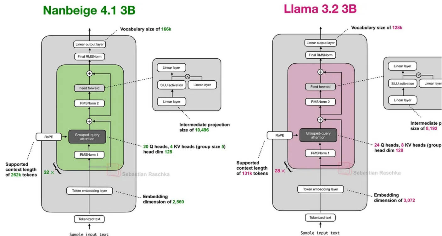
Figure 29: Nanbeige 4.1 3B next to Llama 3.2 3B.
