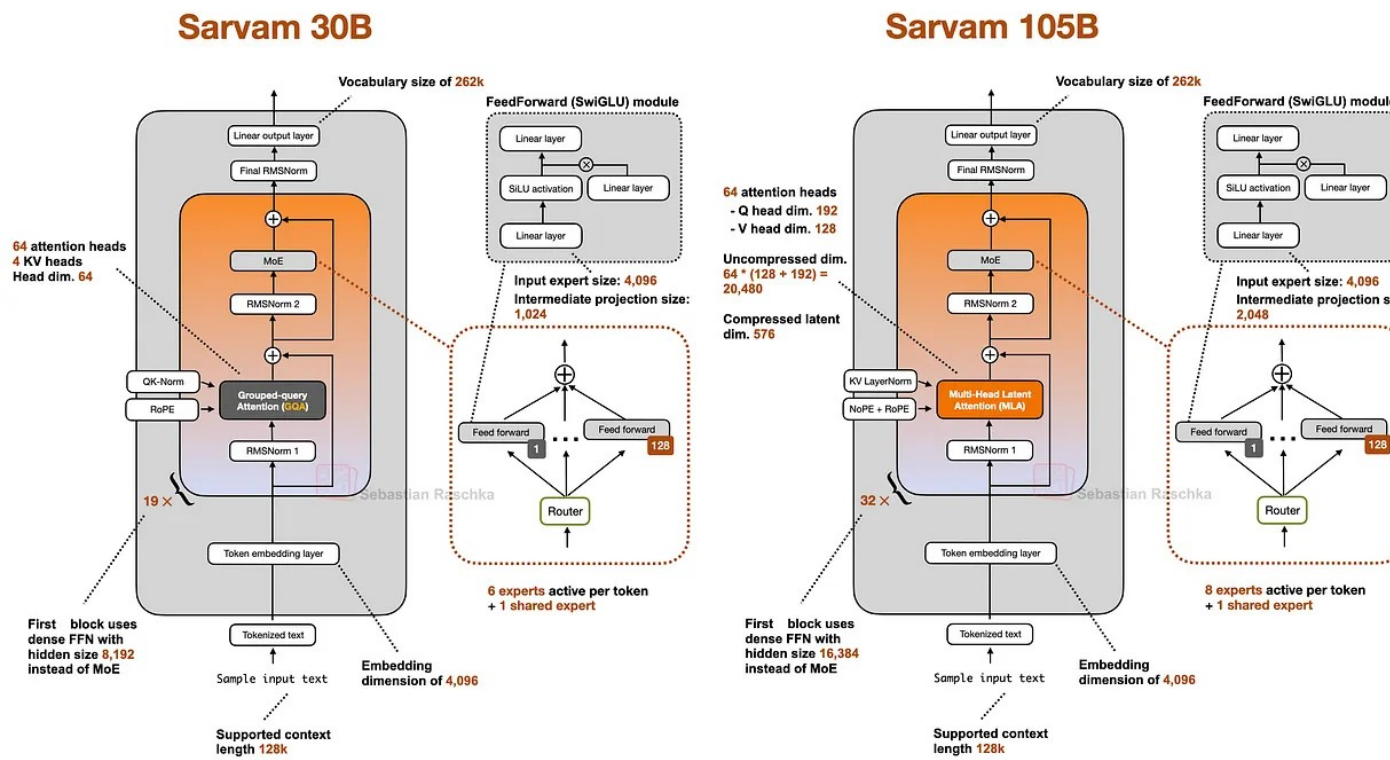
Figure 37: The Sarvam 30B and 105B architectures
