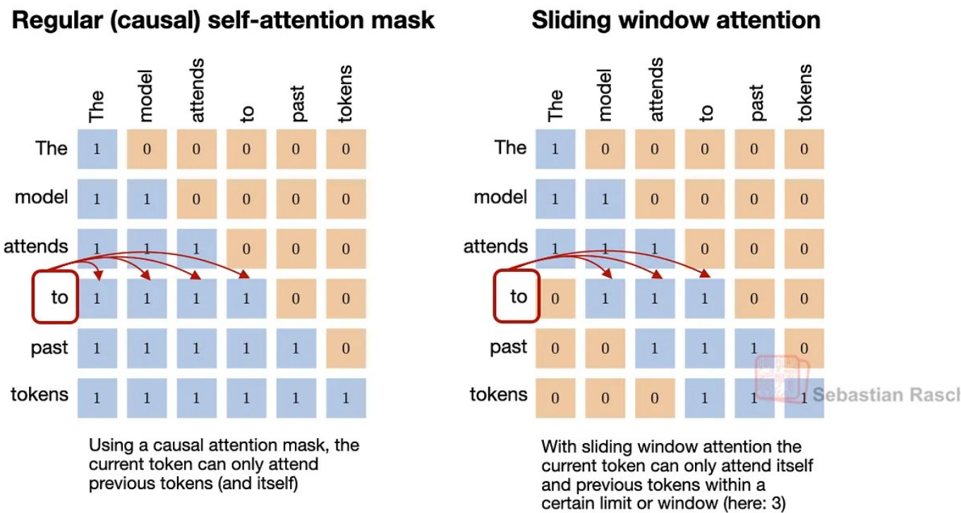
Figure 3: A comparison between regular attention (global attention) and sliding window attention (local attention).
