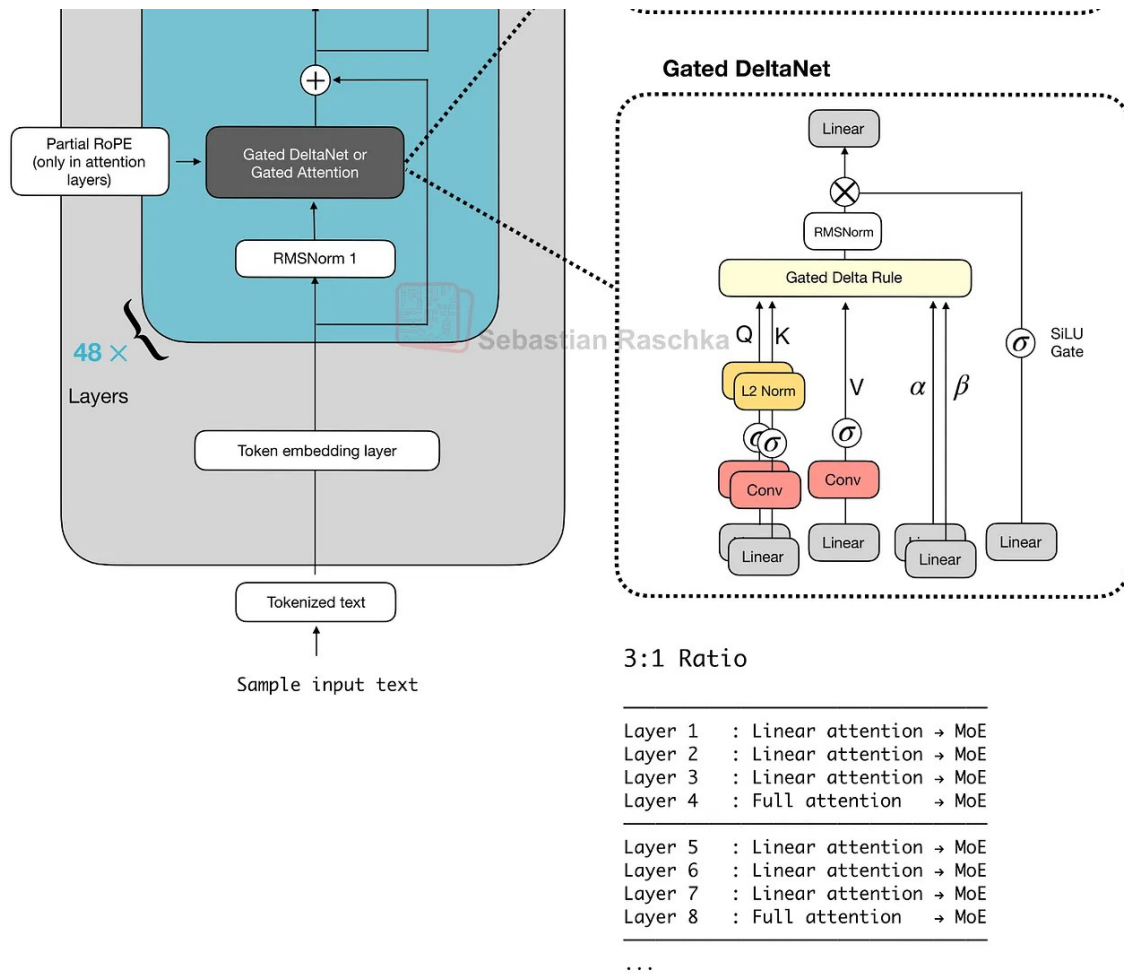
Figure 17: The Qwen3-Coder-Next attention hybrid setup.
