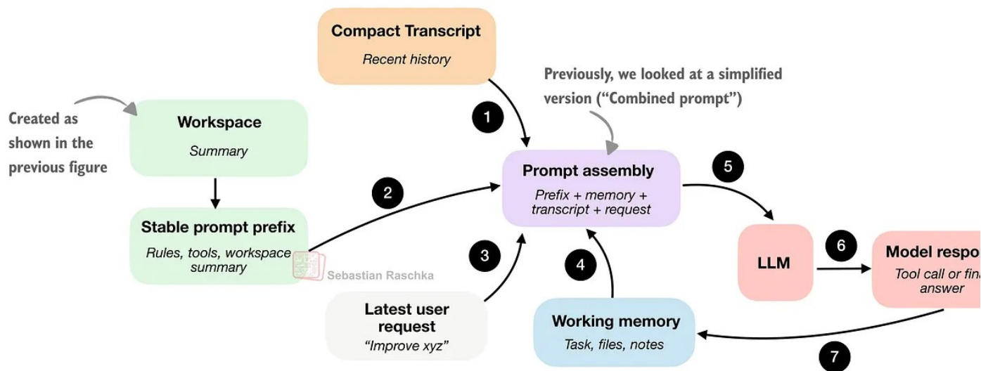
Figure 7: The agent harness builds a stable prompt prefix, adds the changing session state, and then feeds that combined prompt to the model.
