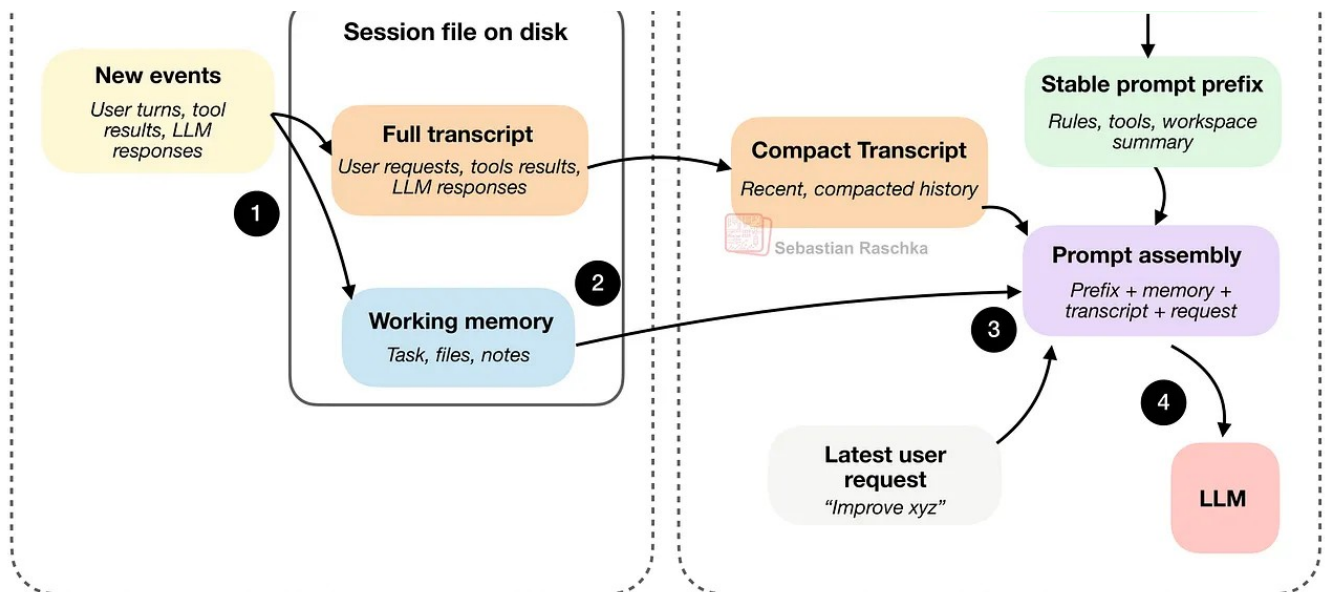
Figure 11: New events get appended to a full transcript and summarized in a working memory. The session files on disk are usually stored as JSON files.
