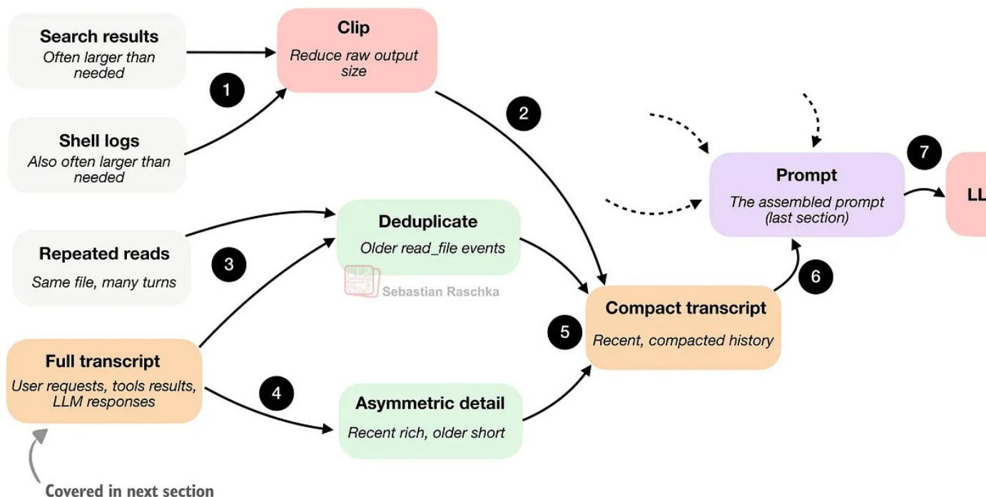
Figure 10: Large outputs are clipped, older reads are deduplicated, and the transcript is compressed before it goes back into the prompt.
