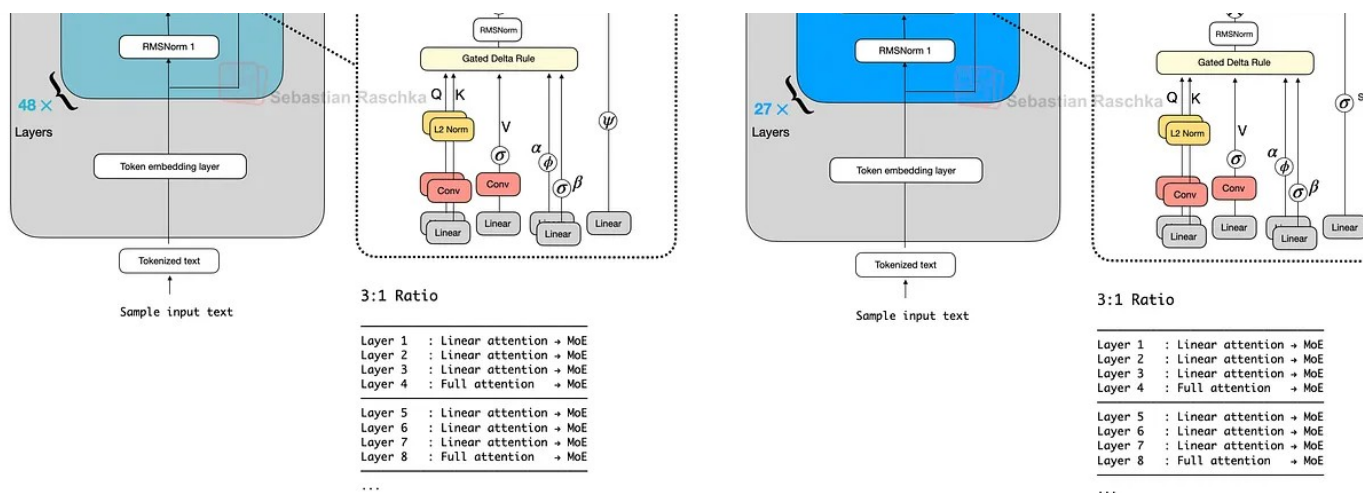
Figure 42: Qwen3-Next and Kimi Linear side by side.
