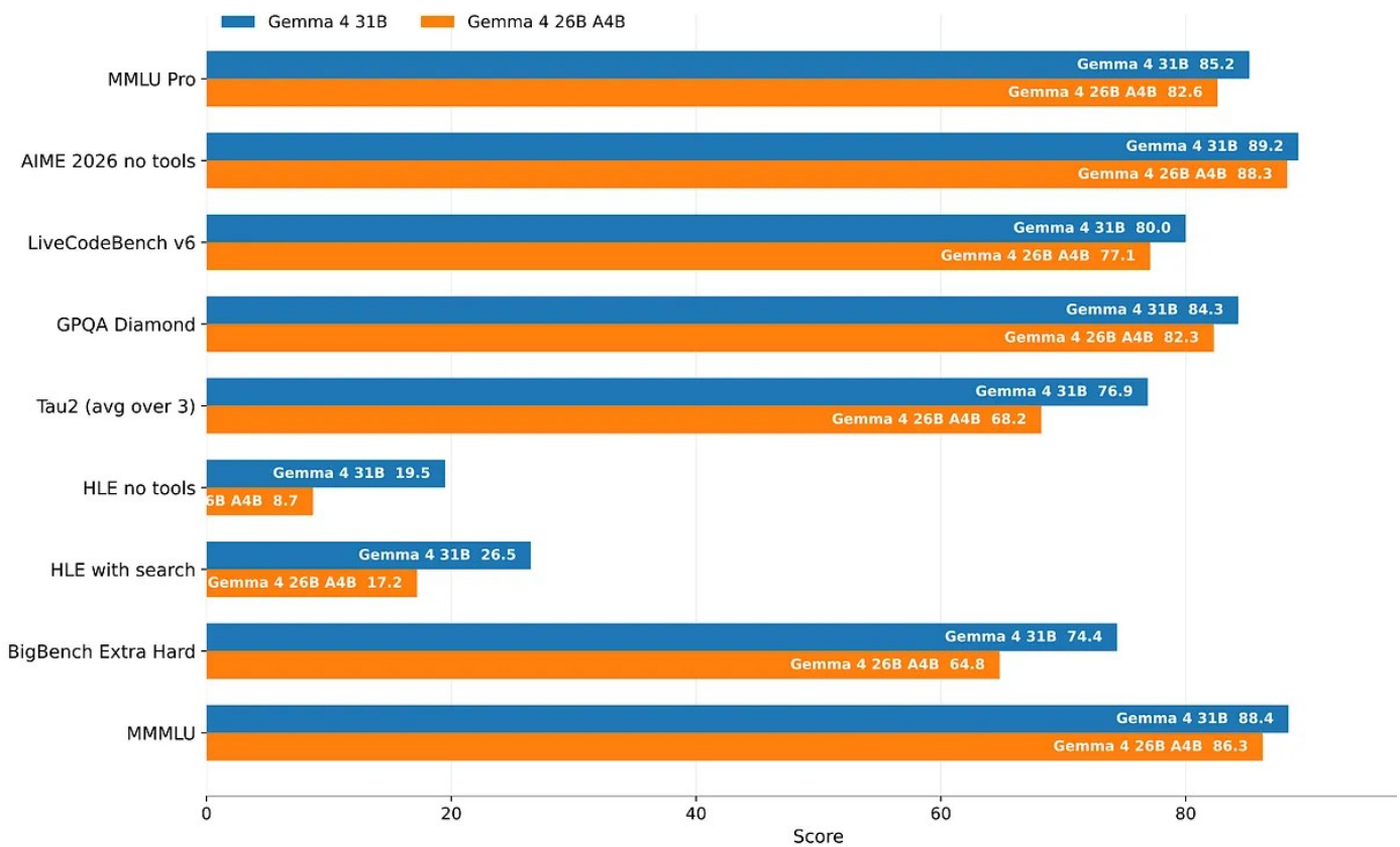
Figure 61: Gemma 4 MoE (26B-A4B) is only slightly worse than Gemma 4 (31B) dense.
