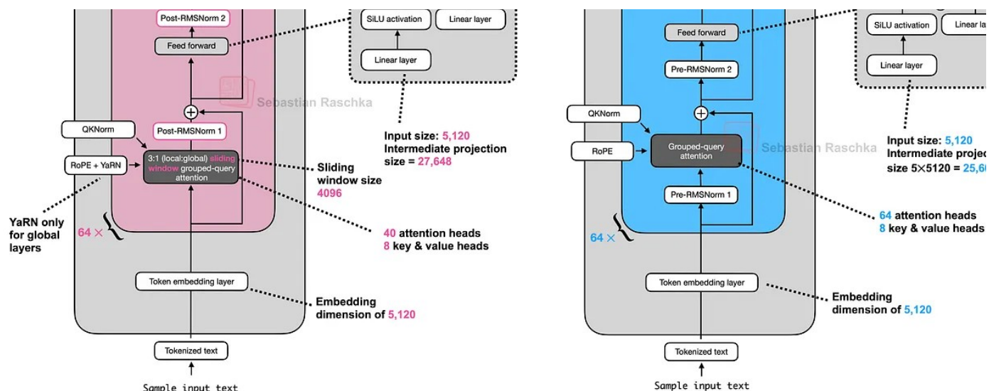
Figure 45: Olmo 3 32B and Qwen3 32B side by side.
