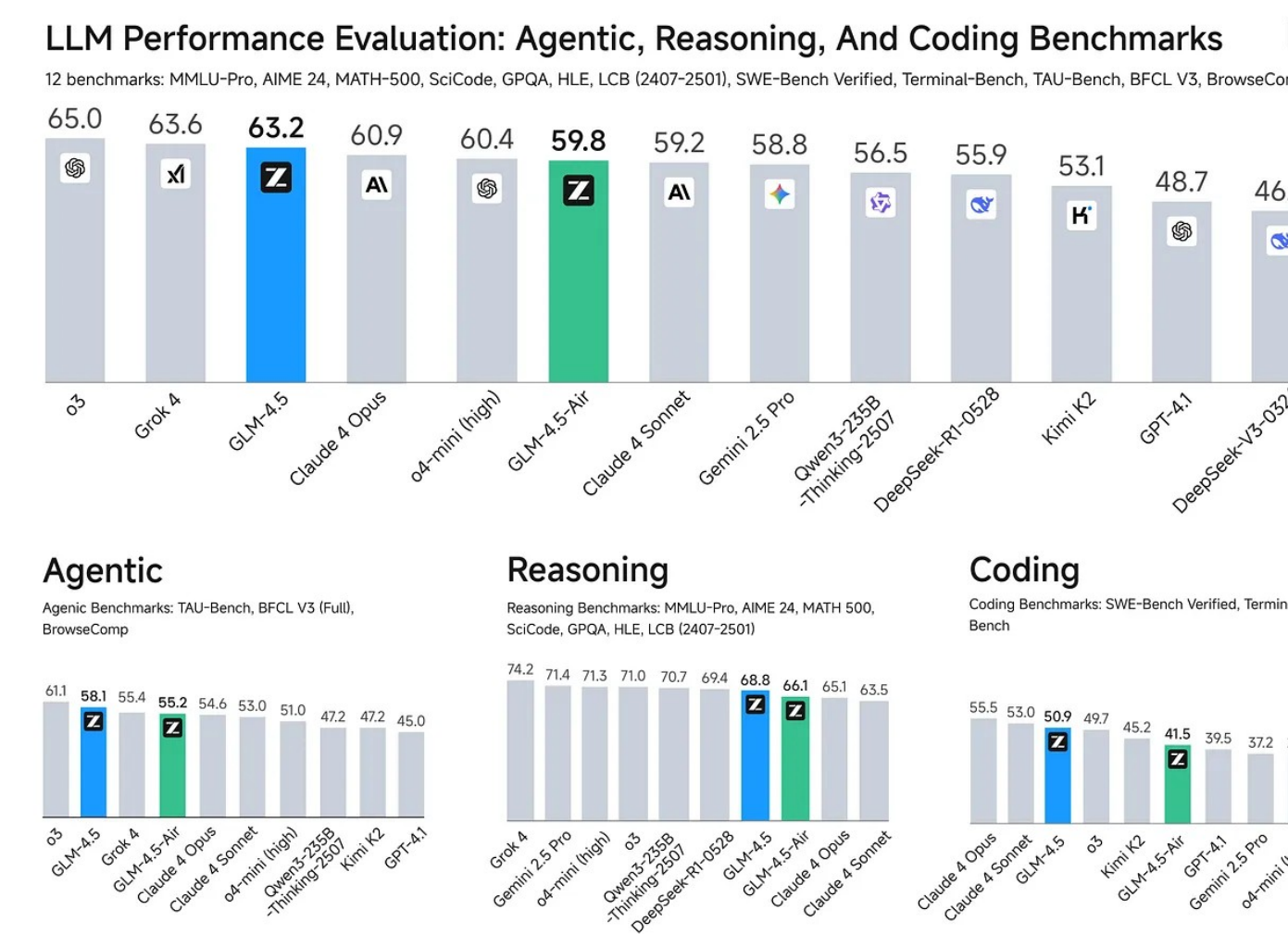
Figure 33: GLM-4.5 benchmark from the official GitHub repository at https://github.com/zai-org/GLM-4.5
