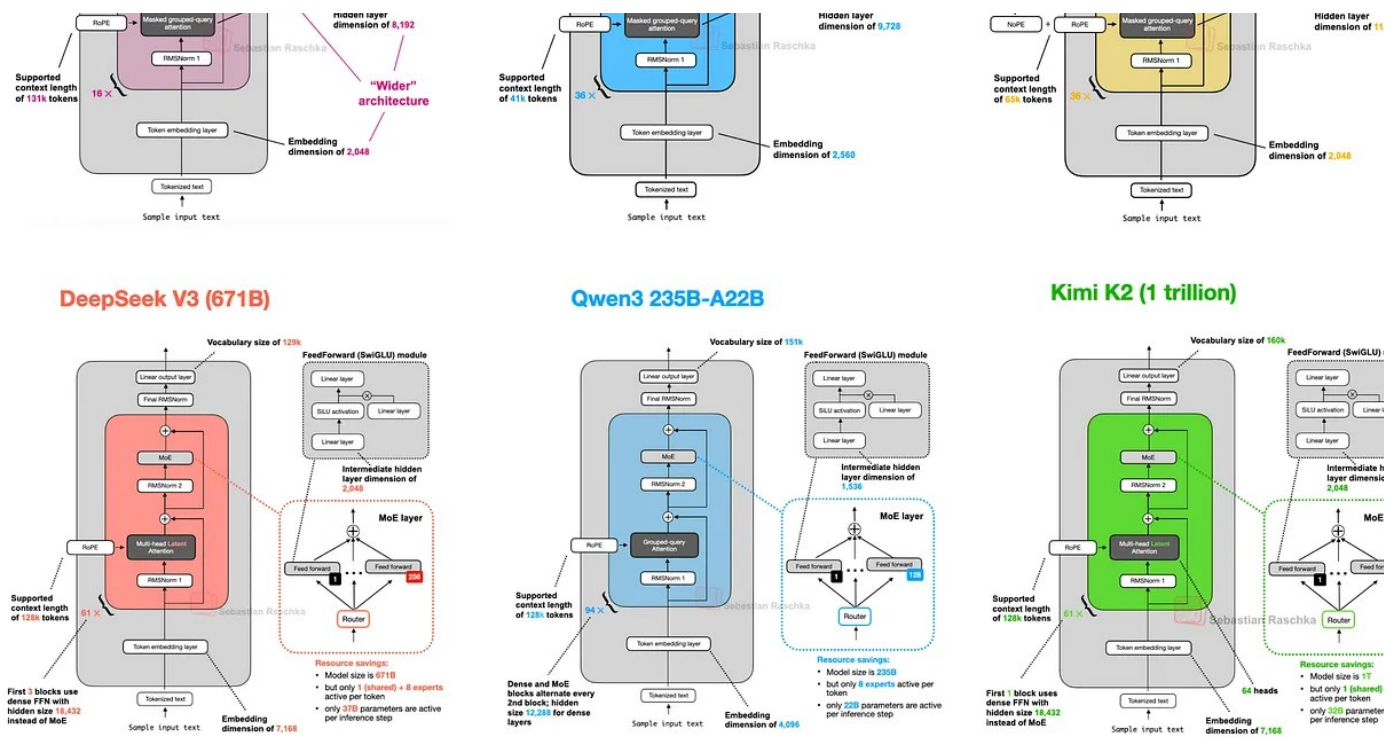
Figure 1: A subset of the architectures covered in this article.
