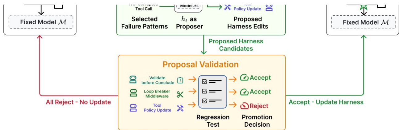
Figure 15: Self-Harness uses a loop of weakness mining, bounded harness proposal, and validation to update a harness. (Image source: Zhang et al. 2026 )
