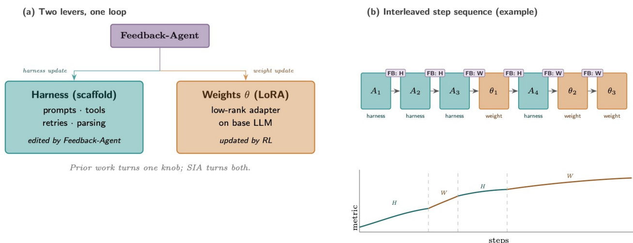
Figure 18: The Feedback-Agent in SIA decides the next iteration type.
