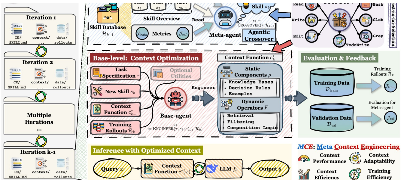
Figure 4: The framework of Meta Context Engineering (MCE): meta-level skill evolution searches over context-management mechanisms, while the base level optimizes the task context. (Image source: Ye et al. 2026)
