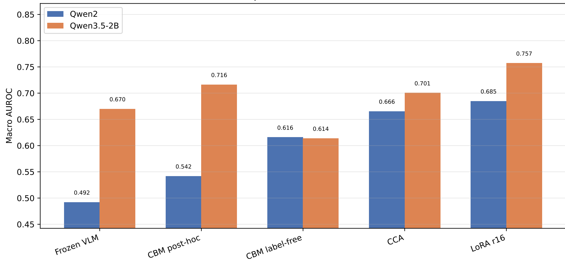
CheXpert test — Macro AUROC
