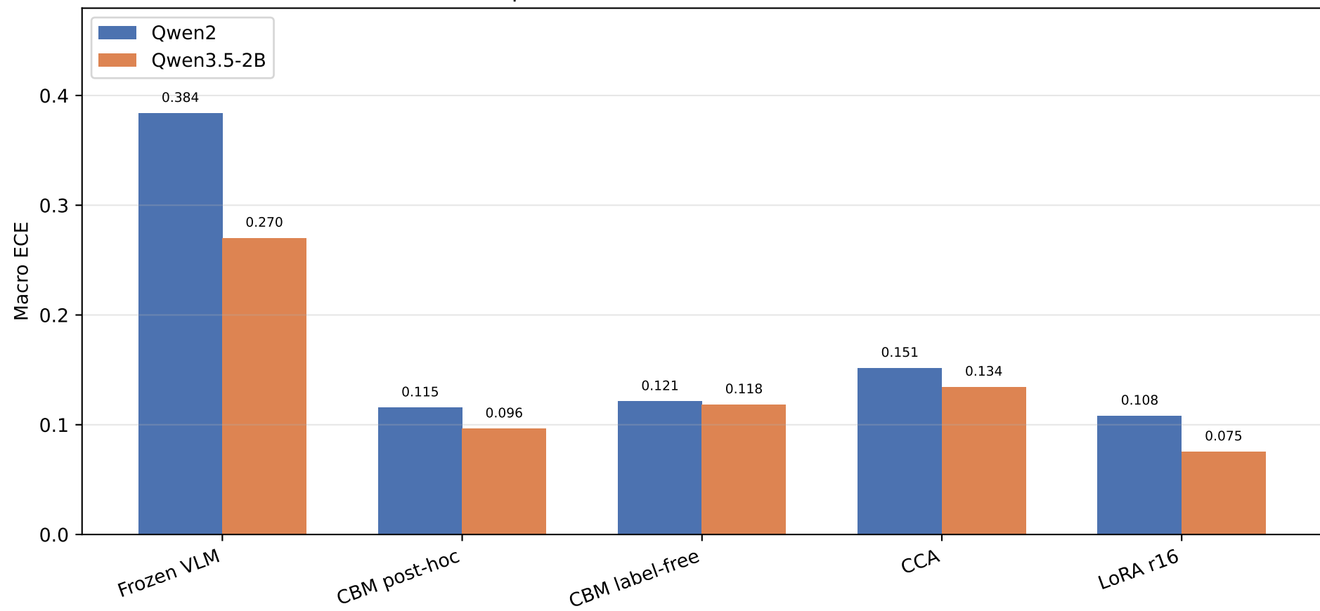
CheXpert test — Macro ECE (lower is better)
