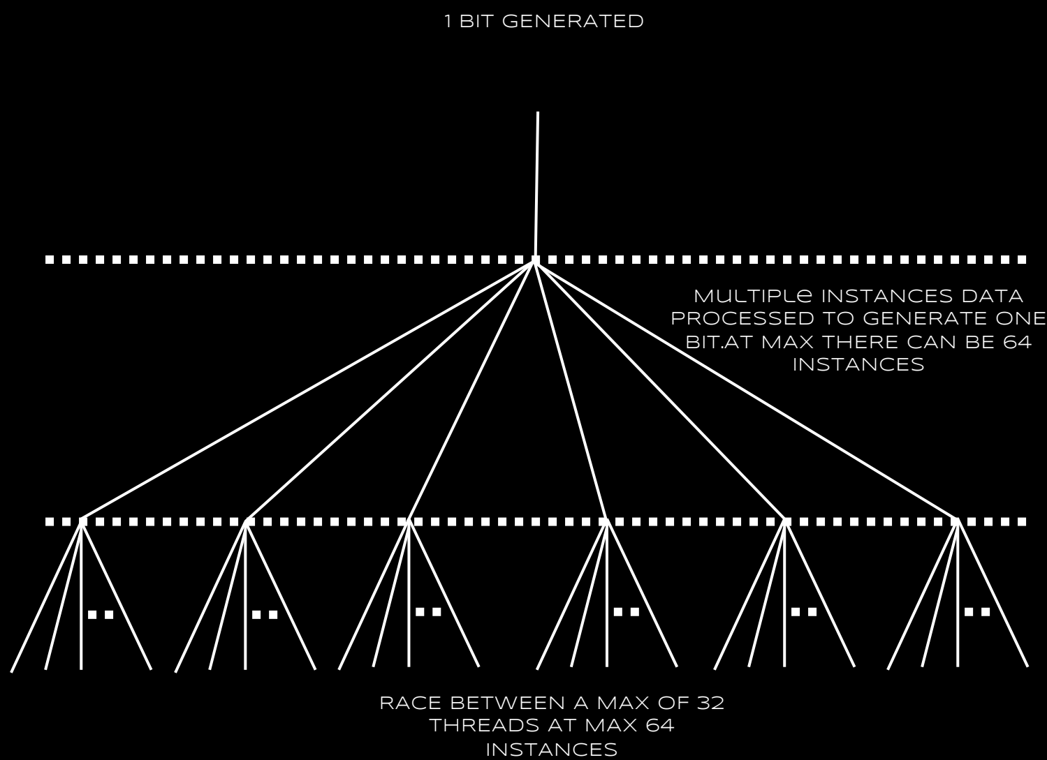
sys-eng/001 – Bit-Based-Randomized-Entropy-System - Scheduler-Based RNG
