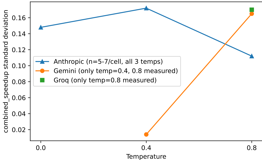
Output Variance vs. Temperature, by Provider
