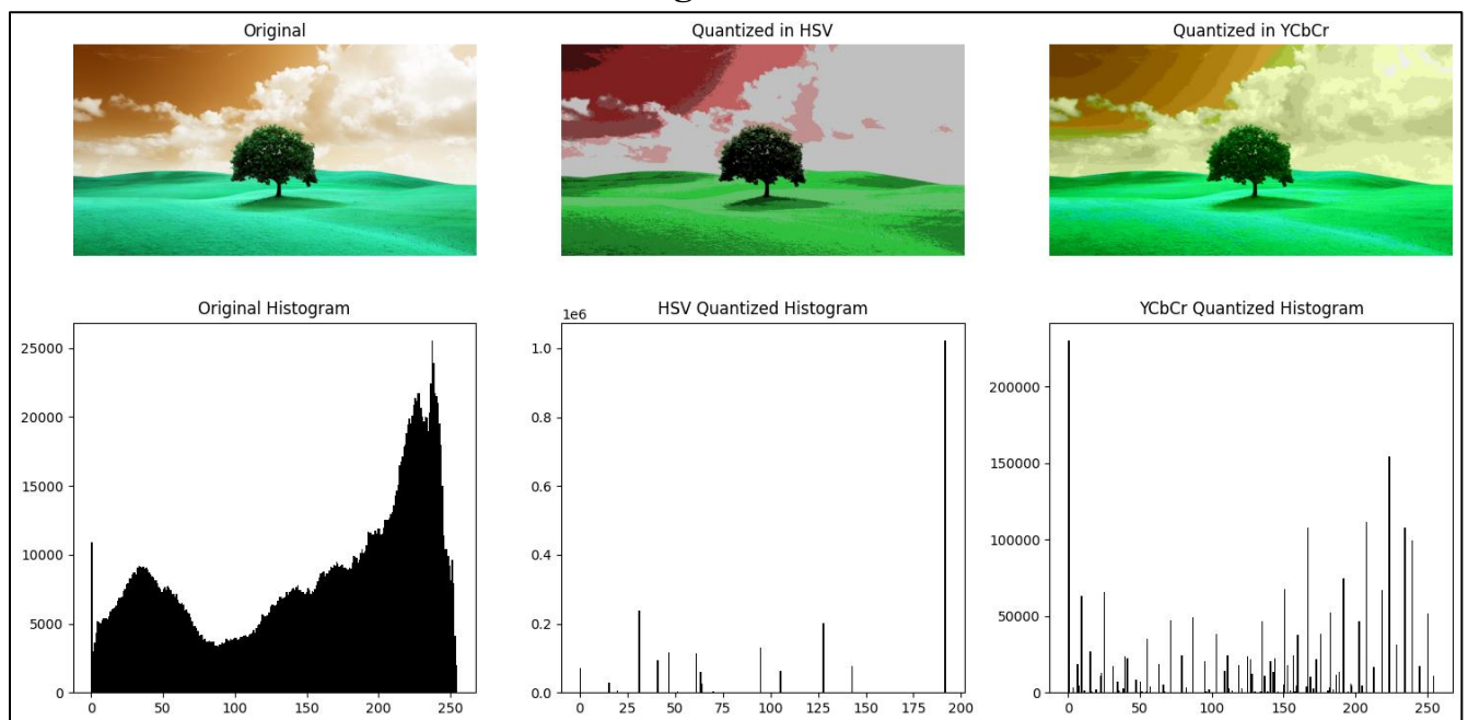
Fig. Color Model Quantization
