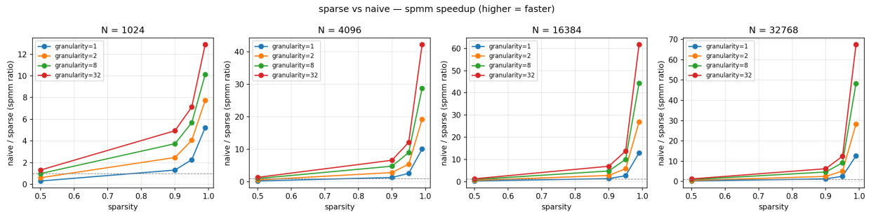
Figure 6: End-to-end speedup of the sparse SpMM kernel over the dense baseline, swept across N , G , and p .
