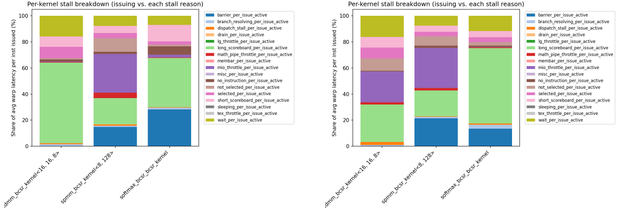
(a) Per-kernel warp stall reasons for N = 1024 .
