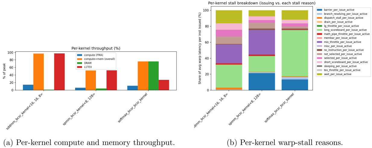
Figure 3: Nsight Compute traces for a N = 32768 , G = 8 , p = 0.95 run. SDDMM and SpMM under-use DRAM bandwidth because most of their loads land in shared memory, while the sparse softmax shows noticeably higher global-memory traffic. The right panel attributes per-kernel stalls: long_scoreboard flags warps waiting on global-memory loads, and mio_throttle flags warps waiting on shared-memory loads.
