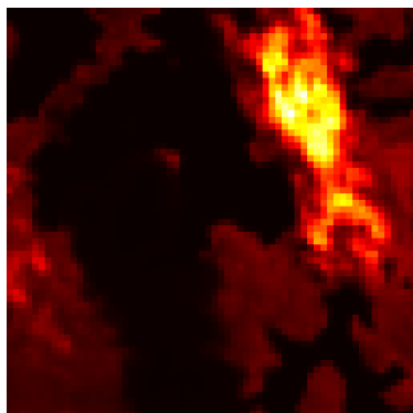
kriging (EQM)
