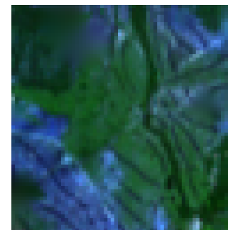
rbf
