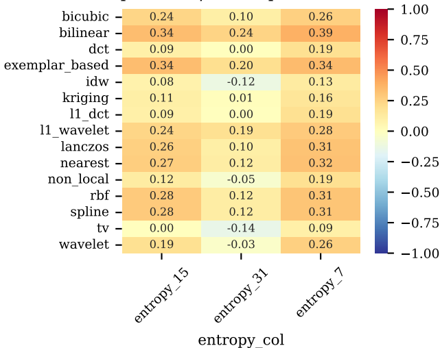
Spearman \rho : Entropia vs PSNR
