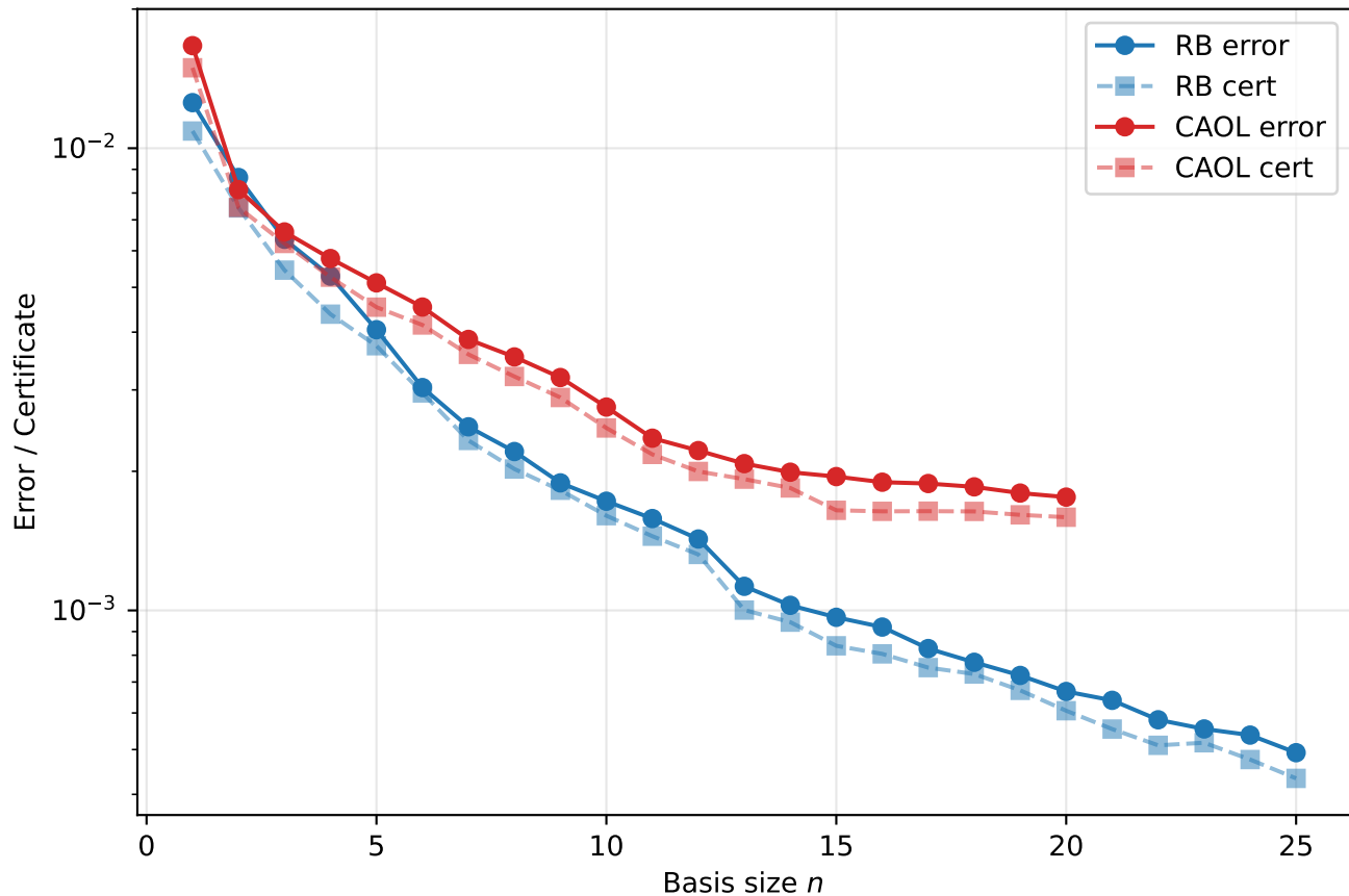
RB vs CAOL: Convergence on 2D affine diffusion
