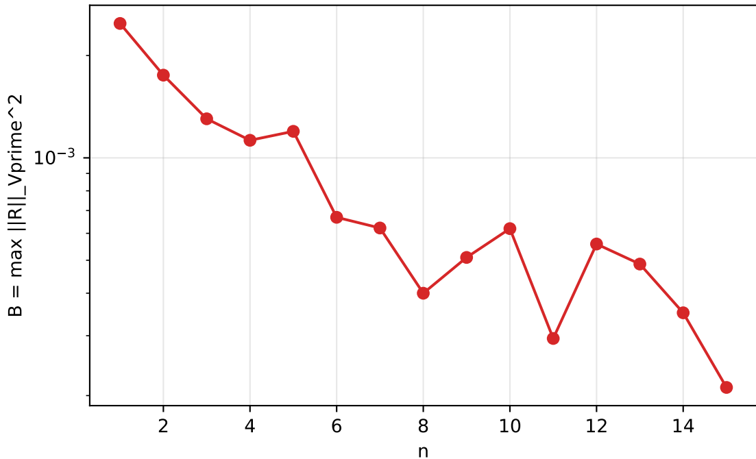
Slow KL ( k^{-0.6} ): residual bound B
