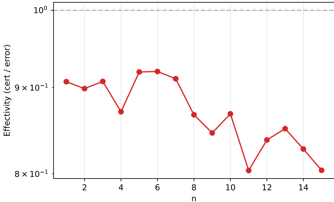
Slow KL ( k^{-0.6} ): effectivity
