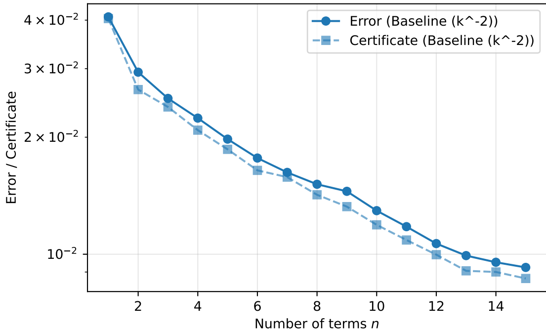
Baseline ( k^{-2} ): error and certificate
