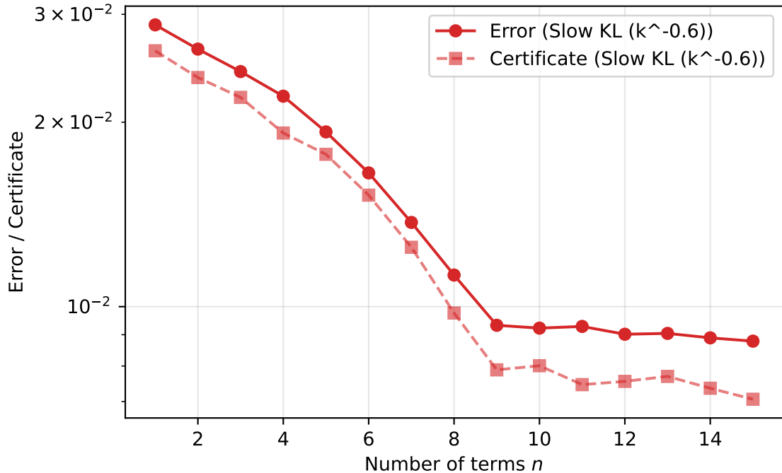
Slow KL ( k^{-0.6} ): error and certificate
