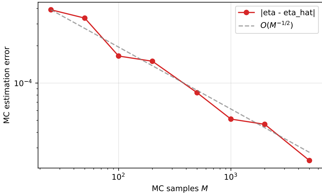
Slow KL ( k^{-0.6} ): MC certification
