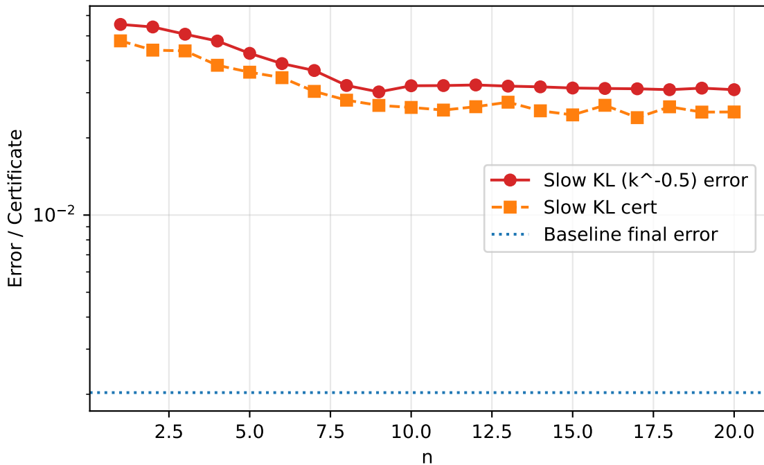
Negative regime: slow KL decay
