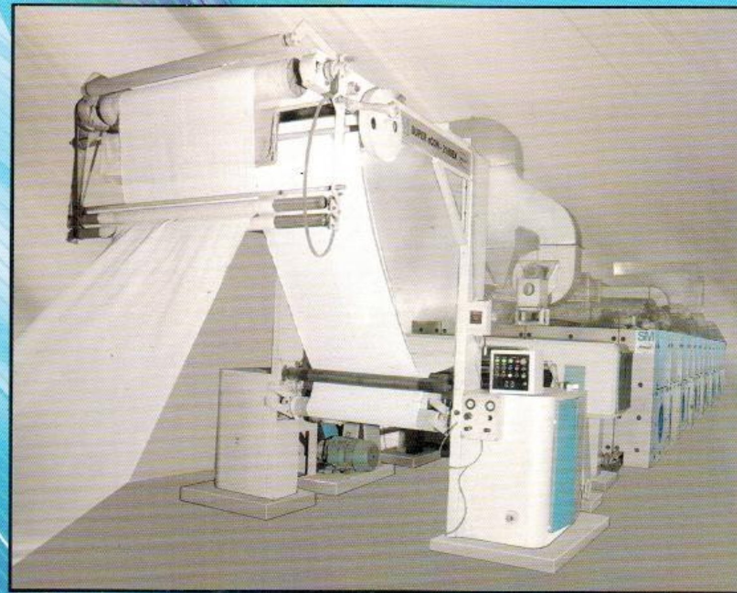
SM HIMSON HOT AIR STENTER MODEL "SUPER e-CON 2200"
