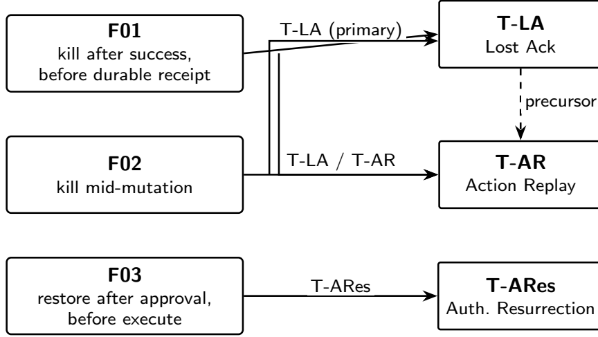
Black/white journal figure. Catalog F01–F03 mapped to ACRFence threats T-LA, T-AR, T-ARes (paper fault-catalog table).
