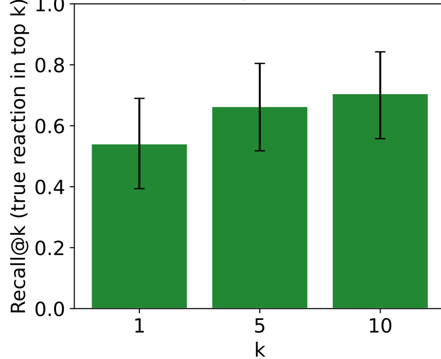
(c) Top-k recall
