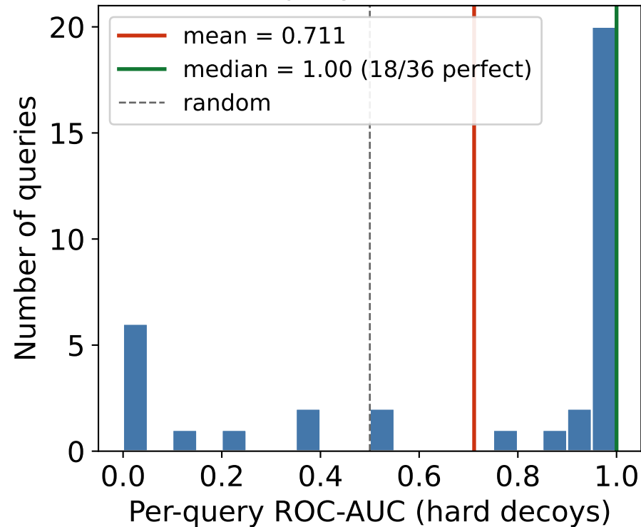
(b) Per-query discrimination
