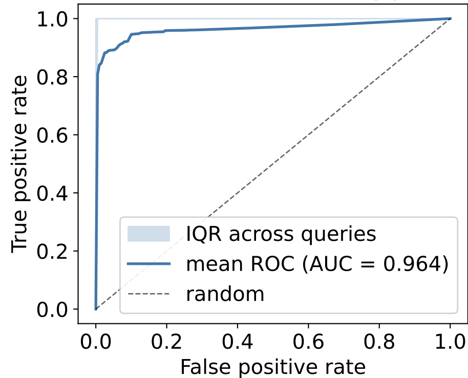
(a) Mean ROC — full decoy pool
