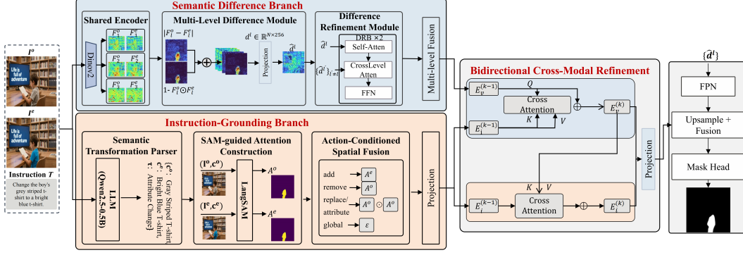
Figure 2: Overview of the SIGMA architecture.
