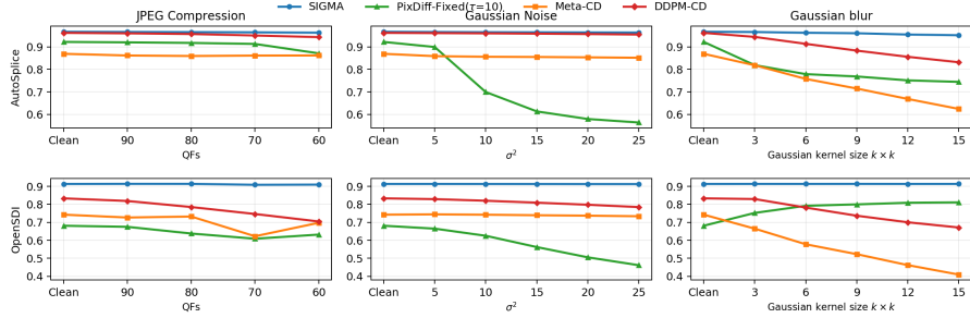
Figure 4: Evaluation of the robustness of SIGMA and comparative baseline methods to JPEG compression, additive white Gaussian noise, and Gaussian blurring on the AutoSplice and OpenSDI datasets.
