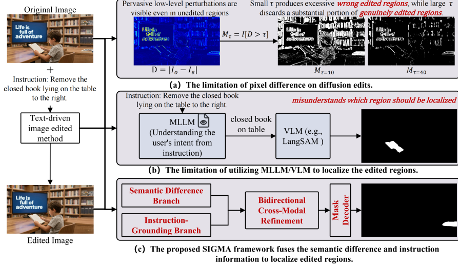
Figure 1: (a) Failure modes of pixel-level differencing under diffusion-based text-driven editing. (b) Failure modes of MLLM/VLM-based mask inference from instructions. (c) Overview of the SIGMA framework.
