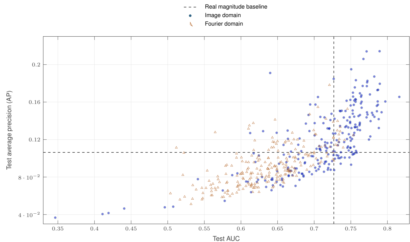
Figure 1: Joint distribution of test AUC and average precision across the 480 complex-valued configurations. Image-domain and Fourier-domain configurations are distinguished by marker style; dashed reference lines denote the fixed real magnitude baseline in AUC and average precision.
