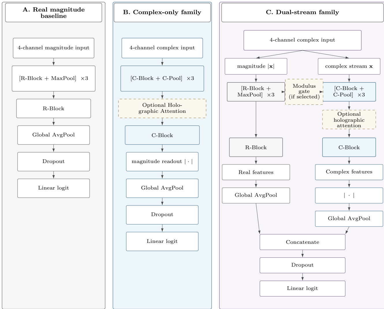
Figure 3. High-level model families evaluated in the study. The real baseline processes coil magnitudes, the complex-only family retains complex-valued features until magnitude readout, and the dual-stream family processes magnitude and complex representations in parallel before feature fusion. Repeated processing stages are shown using \times 3 notation.
