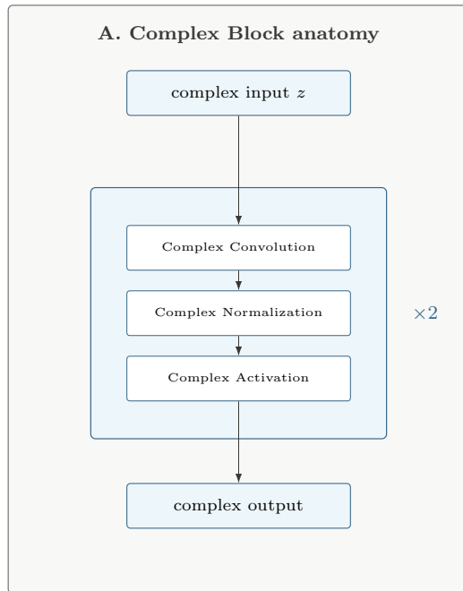
Figure 4. Complex Block anatomy showing two repeated convolution–normalization–activation sequences from complex input to complex output.
